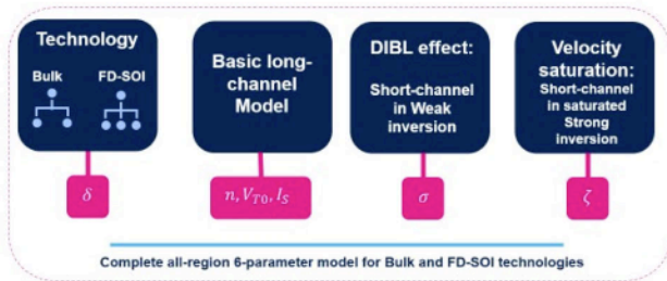
FIGURE 7. Conceptual structure of the ACM2 MODEL.
