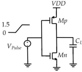
FIGURE 14. Schematic of the inverter.
