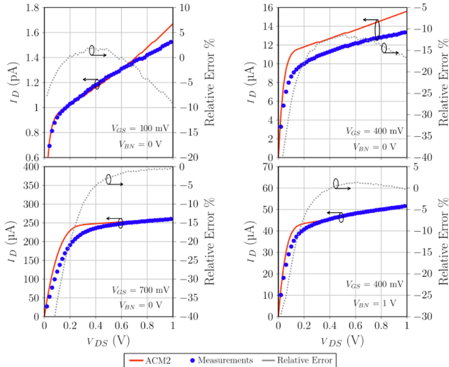
FIGURE 11. I_D - V_D Characteristics for a NMOS LVT transistor from the 28 nm FD-SOI CMOS technology with W/L = 1 \mu\text{m}/60 \text{ nm} for different V_{GS} and V_{BN} .
