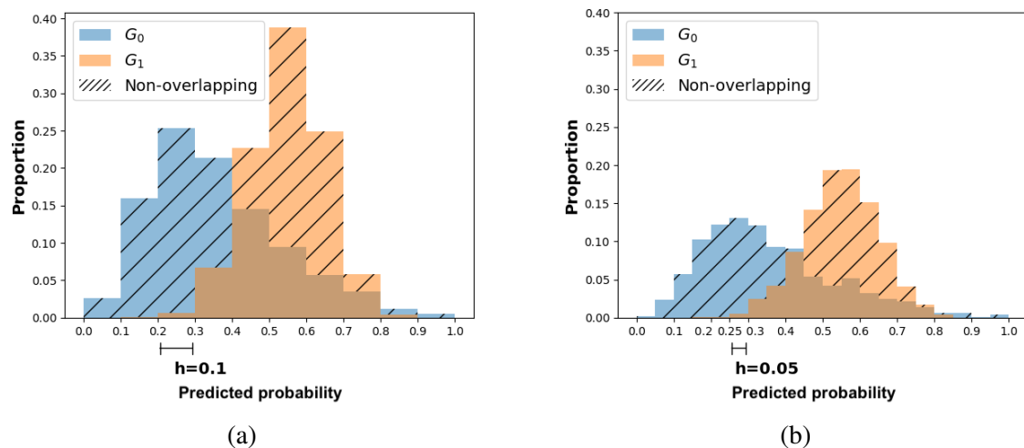
Figure 5: Visual representation of the influence of the bandwidth h on MADD.
