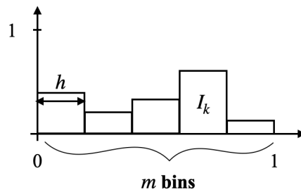
Figure 1: Illustration of the notations introduced for MADD.
