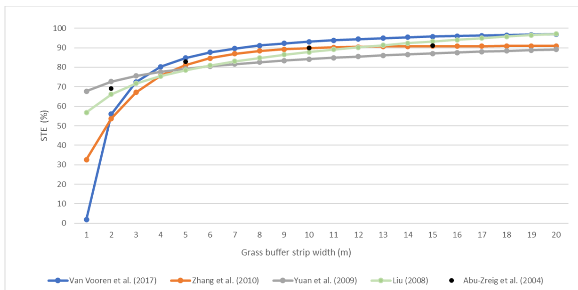
Figure 1: Sediment trapping efficiency (STE) in function of grass buffer strip width (m)
