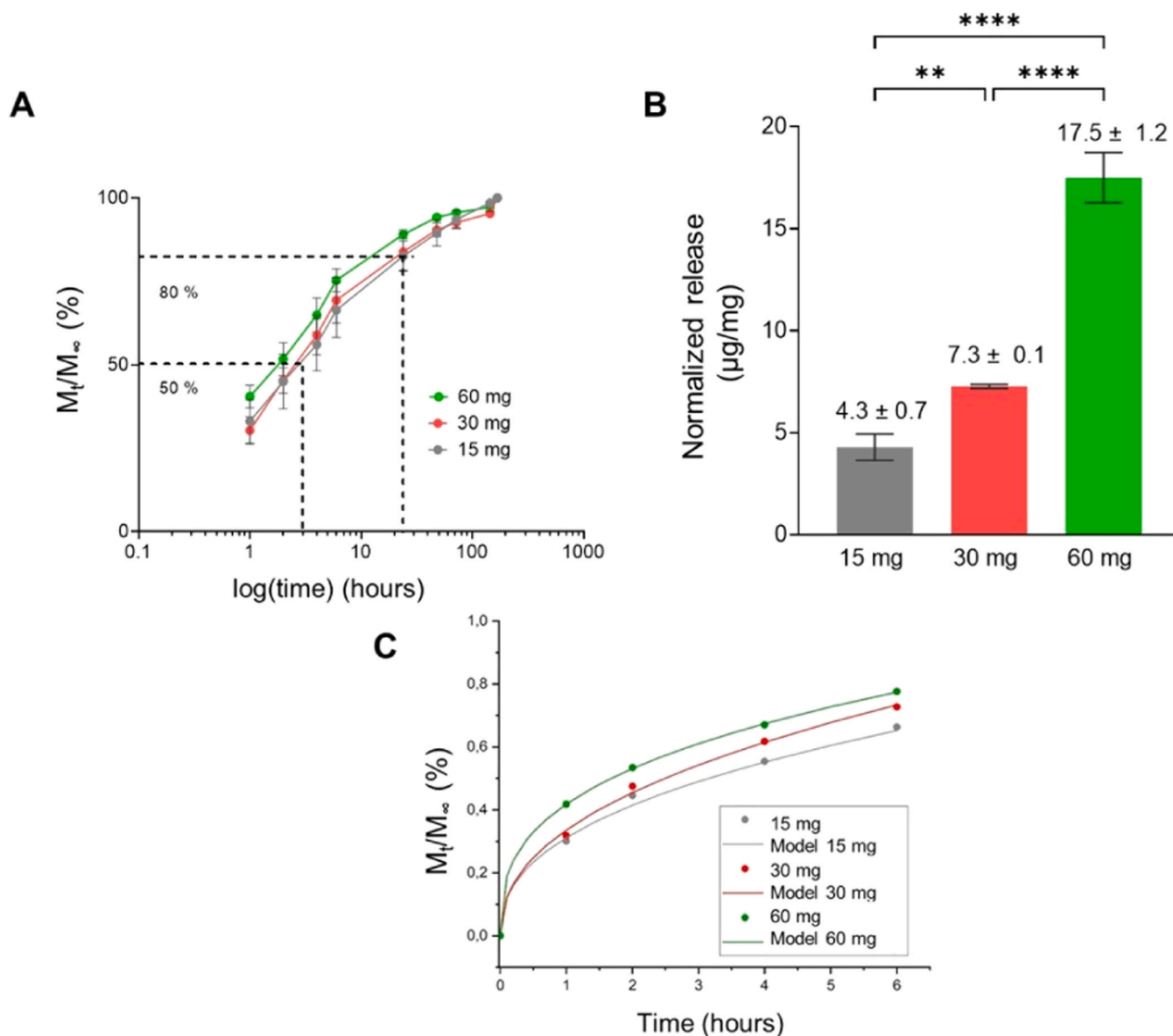
Fig. 4. A- Time-dependent release curves of prednisolone at 37°C presented as percentage of cumulative release M_t on total release M_\infty using increasing initial quantity in loading ethanol buffer 15 mg, 30 mg and 60 mg. B- Total normalized release of prednisolone from bilayers using ethanol loading solution containing 15 mg, 30 mg, and 60 mg (bilayers thickness 241 \pm 26 \mu\text{m} , values are expressed as mean \pm SD, n=3 , one-way ANOVA with Tukey post hoc test, ** p < 0.01 , **** p < 0.0001 ). C- Fit of the Korsmeyer-Peppas model to experimentally determined prednisolone release kinetics from copolymers-based films on first 60 % of released solute (curve= model, symbols=experiment).
