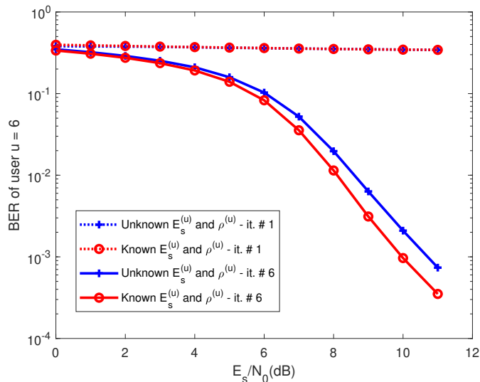
Fig. 15. BER under unknown hyperparameters - low energy user u = 6 .
