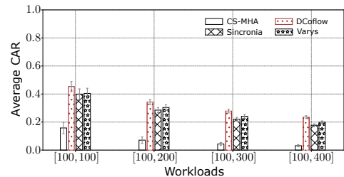
(b) Synthetic traffic traces on large-scale networks.
