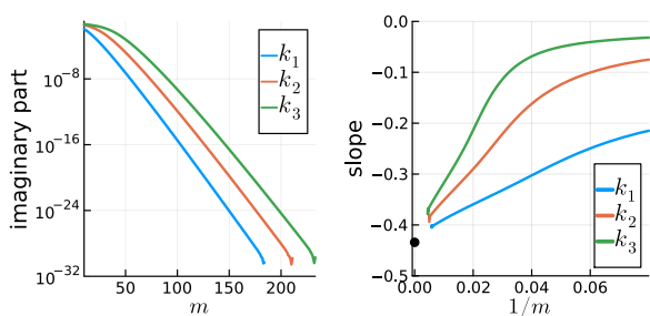
Figure 5: Left, \text{Im } k_j(m) vs m . Right, the slope \log |\text{Im } k_j(m+1)| - \log |\text{Im } k_j(m)| vs 1/m , expected to converge to -2S_0 (marked with \bullet ), cf (10).
