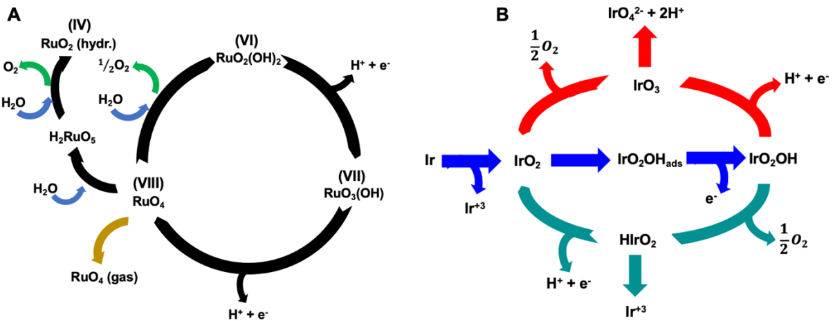
16 17 Fig. 11. (A) Depiction of the Ru metal oxidation state during the oxygen evolution and corrosion processes on Ru and 18 RuO 2 electrodes reproduced from Kötzt et al. [131] (B) Ir dissolution scheme at higher anode potentials indicated in red
