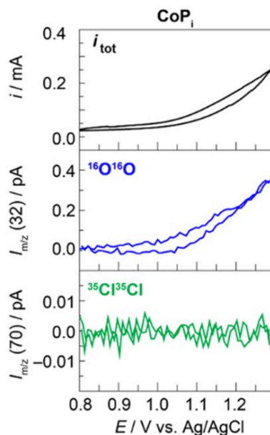
1 2 Fig. 36. The top panel is a cyclic voltammogram of CoP i in an aqueous solution of 100 mM KP i and 500 mM NaCl at a 3 scan rate of 5 mV/s. The middle and bottom panels are the DEMS results for the evolved oxygen and the evolved 4 chlorine, respectively. Figure of Kean and Nocera [238].
