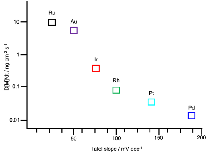
1 2 Fig. 10. A scatter plot of the dissolution rate at j = 5 mA cm -2 determined through scanning flow cell/inductively coupled 3 plasma mass spectrometry as a function of the Tafel slope taken from ohmic drop compensate current-potential curves 4 scanned at 2 mV s -1 . Reproduced from Cherevko et al. [129].
