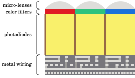
Fig. 4. Structure of a back-side illumination pixel
