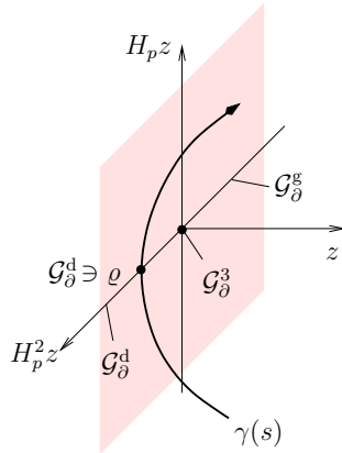
FIGURE 5. A bicharacteristic going through a diffractive point ( \mathcal{G}_\vartheta^d ).
