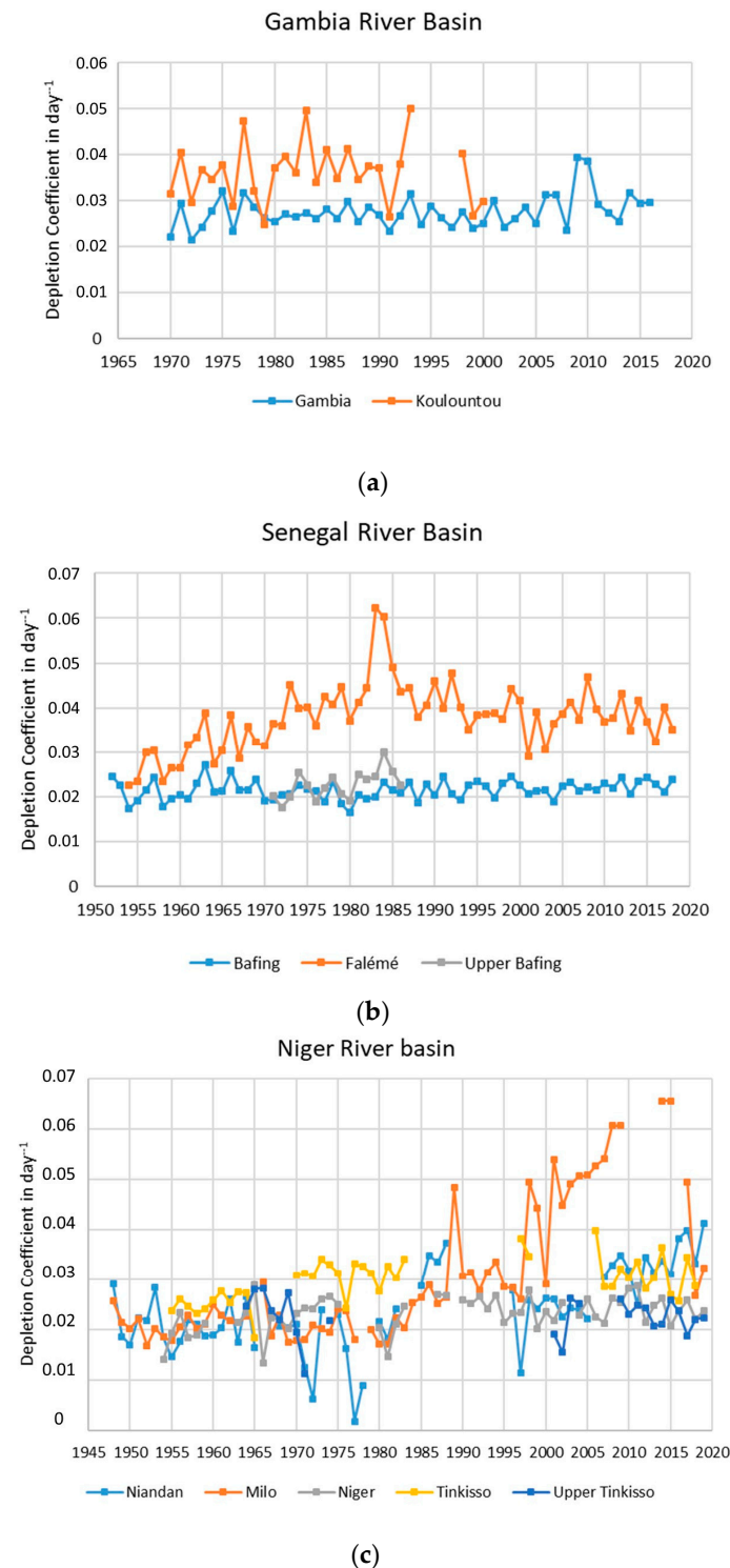
Figure 7. Evolution of depletion coefficients of rivers in Gambia (a), the Senegal (b), and the Niger River Basin (c) since the 1950s [17].
