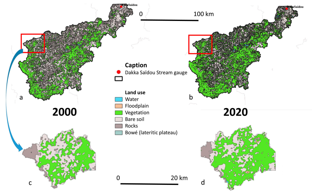
Figure 11. Vegetation evolution in green color, between 2000 ((a,c) panels) and 2020 ((b,d) panels), in the Bafing basin ((a,b) panels) (Guinea, name of the Upper Senegal River basin), and zoom on the area of Labé ((c,d) panels) (the major city of the range), the most densely populated area [69] (The grey sector westward is the suburbs of Labé).
