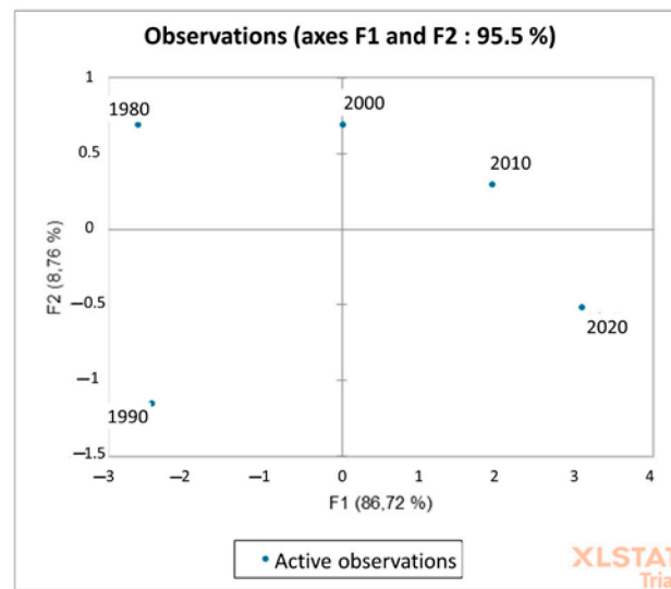
Figure 10. Distribution of samples in their statistical space.
