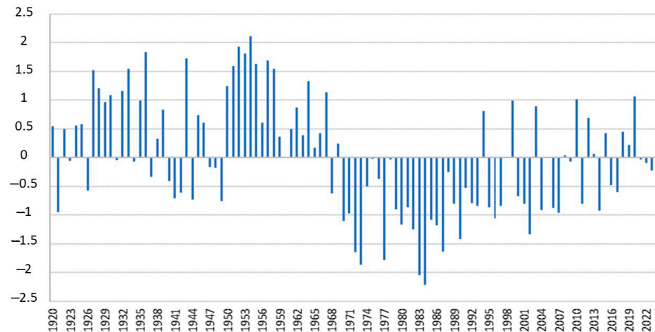
Figure 2. Standard precipitation index from 1920 to 2020 in the whole West African Sahel.
