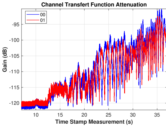
Fig. 5. The gain of the CTF during the measurement. In blue, for the first channel from the antenna on top of the front-end and in red for the second channel from the antenna below.
