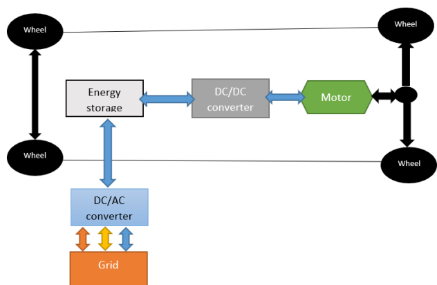
Figure 5: Electric Vehicle Battery pack with Grid Connection
