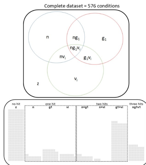
Figure 5. (top) Schematic representation of the comparison of three datasets: Dataset( N^{cum} ) in blue, dataset( G_1^{cum} ) in red and Dataset( V_i ) in green defining the 8 sub-categories ( z , n , g_1 , v_i , ng_1 , g_1v_i , nv_i and ng_1v_i ). (bottom) Example of the SOI analysis ( v_i = v_1 ) generated by our home-made database, enabling the comparison of cumulated HEWL native ( N^{cum} ), cumulated HEWL–Tb–Xo4 ( G_1^{cum} ) and HEWL-variant V_1 datasets.
