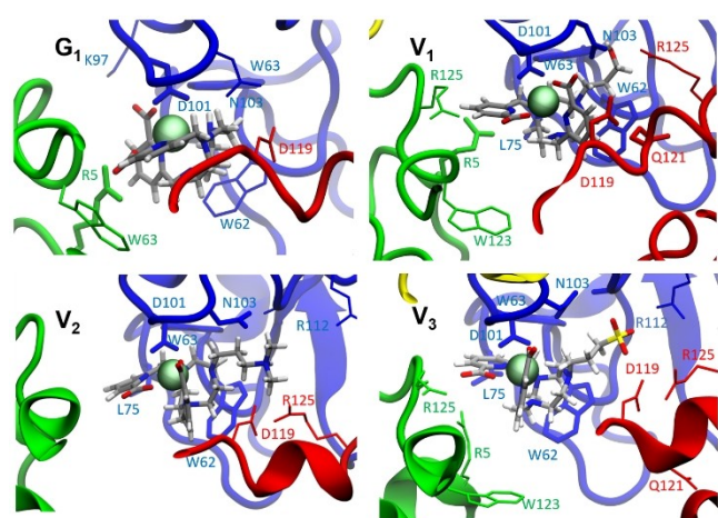
Figure 8. Binding pocket of G_1 and the three variants V_1 , V_2 and V_3 at the interface of the four HEWL (blue: HEWL A; red: HEWL B; green: HEWL C; yellow: HEWL D). Yttrium cation is represented by the green sphere, ligand and interacting residues (Occurrence rate > 0.5 ) are drawn with ball and stick representations.
