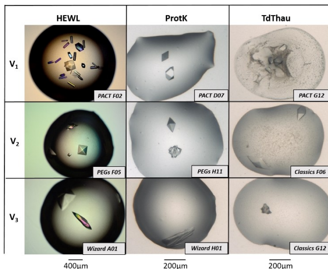
Figure 4. Pictures of [protein/ V_i ] co-crystals using either Olympus microscope under polarized light or from the HTX imaging system. Crystallization kit and condition in italic.
