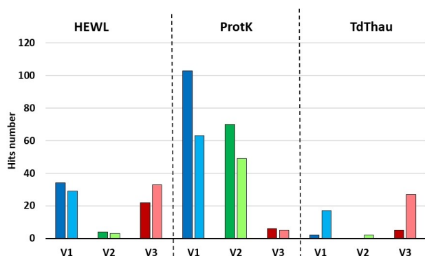
Figure 6. Analysis of the complementary hit number for each variant compared to G_1 with the three model proteins HEWL, protK and TdThau. The dark colored part indicates the 6 score (mono-crystal) and the light colored one, the additional 4 and 5 scores (needle, urchin and micro-crystals).
