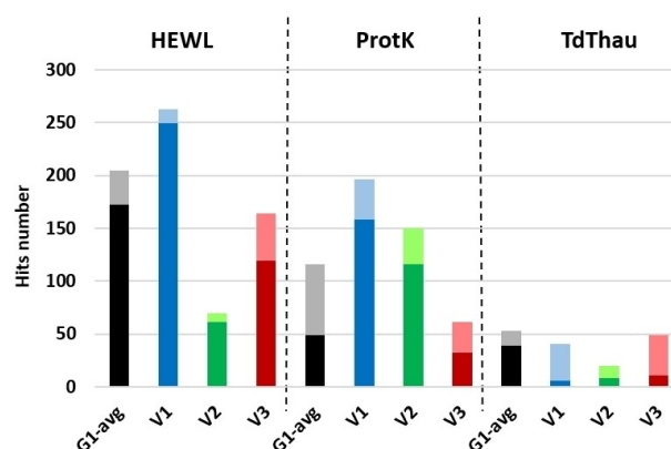
Figure 3. Analysis of the hit number of the automated crystallization experiments performed with the different additives and the three model proteins HEWL, protK and TdThau. The dark colored part indicates the 6 score (mono-crystal) and the light colored one, the additional 4 and 5 scores (needle, urchin and micro-crystals).
