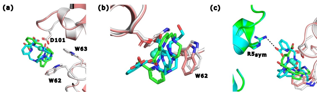
Figure 7. Binding site comparison between Tb–Xo4 (G 1 ) and the variant with propanol pendant arm (V 1 ). (a) Superimposition of interaction sites in {G 1 /HEWL} (in white) and in {V 1 /HEWL} (in salmon). G 1 and V 1 variant molecules are colored in green and cyan, respectively. (b) Different view of (a) showing the change in W62 position. (c) Extra view of the superposition showing the interaction with R5 from a symmetrical molecule. The crystal-symmetry related molecules are colored similarly to their respective lanthanide complexes (green and cyan for {G 1 /HEWL} and {V 1 /HEWL}, respectively). The protein molecules are depicted in cartoon mode with the exception of interacting residues represented as sticks.
