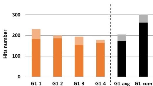
Figure 2. Analysis of the hit number of crystallization experiments with G_1 and HEWL, the average (avg) and cumulated data (cum). The dark colored part indicates the 6 score (mono-crystal) and the light colored one, the additional 4 and 5 scores (needle, urchin and micro-crystals).
