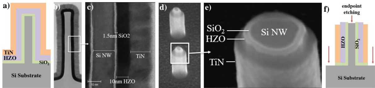
Figure 2 : (a)Schematic of the vertical HZO/TiN deposition. (b) TEM from vertical nanowire with crystallized SiO 2 /HZO/TiN multistack with a (c) zoomed view on the critical sidewall. (d)birds view SEM plasma etched vertical nanowires where TiN/HZO have been removed from (e) top and bottom with the corresponding 2D sketch(f)
