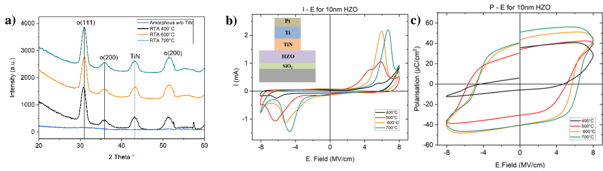
Figure 1: (a) GIXRD verification of the crystalline nature and identification of the orthorhombic phase on our planar samples. The electrical measurements were conducted on a stack of 1.5nm of SiO 2 on Si substrate followed by 10nm of HZO, 13nm of TiN and a total of 35 nm of Ti/Pt as top contact. Results of I vs E field (b) and P vs E field (c) demonstrate the evolution of polarization and Ec for different HZO activation annealing temperatures.
