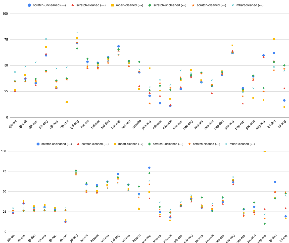
Figure 8: Results on the LegoMT test sets using the models trained on all (top) and public (bottom) data.
