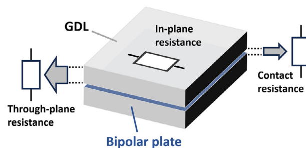
FIGURE 1 | Representation of R_c , through-plane resistance ( R_p ), and in-plane resistance ( R_i ) in the GDL/BPP assembly. BPP, bipolar plate; R_c , contact resistance.
