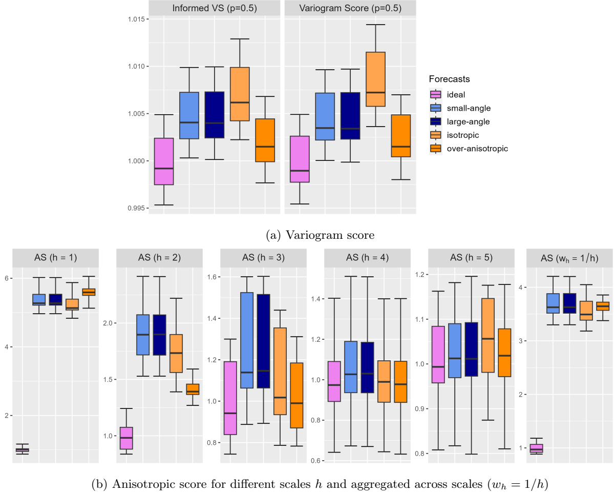
Figure 3: Expectation of interpretable proper scoring rules focused the dependence structure: (a) the variogram score and (b) the anisotropic score, for the ideal forecast (violet), the small-angle forecast (lighter blue), the large-angle forecast (darker blue), the isotropic forecast (lighter orange) and the over-anisotropic forecast (darker orange). More details are available in the main text.
