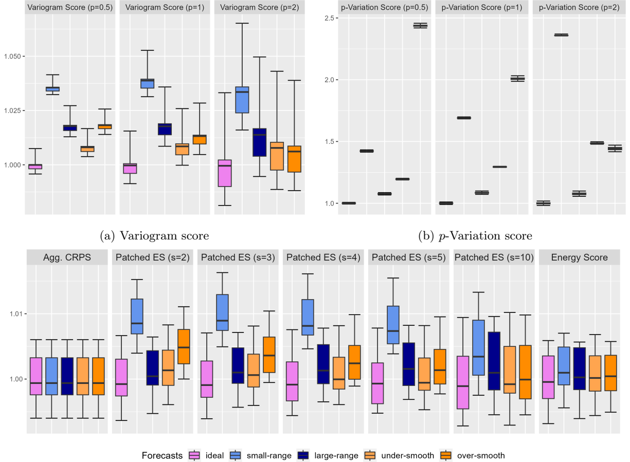
(c) Aggregated CRPS, patched ESs and ES
