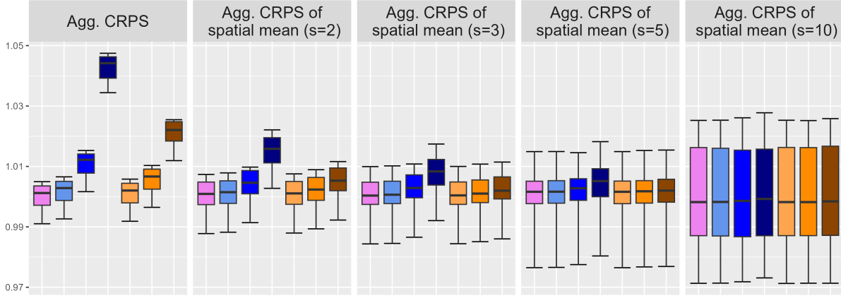
(a) Aggregated CRPS and CRPS of spatial mean
