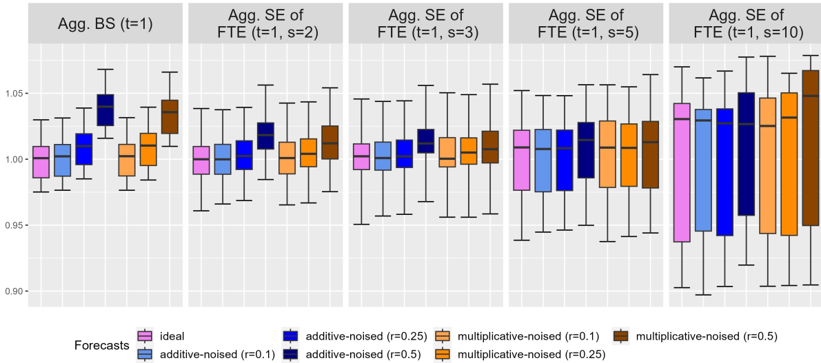
(b) Aggregated BS and SE of FTE
