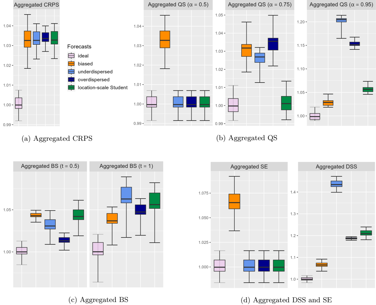
Figure 1: Expectation of aggregated univariate scoring rules: (a) the CRPS, (b) the quantile score, (c) the Brier score, and (d) the squared error and the Dawid-Sebastiani score, for the ideal forecast (light violet), a biased forecast (orange), an under-dispersed forecast (lighter blue), an over-dispersed forecast (darker blue) and a local-scale Student forecast (green). More details are available in the main text.
