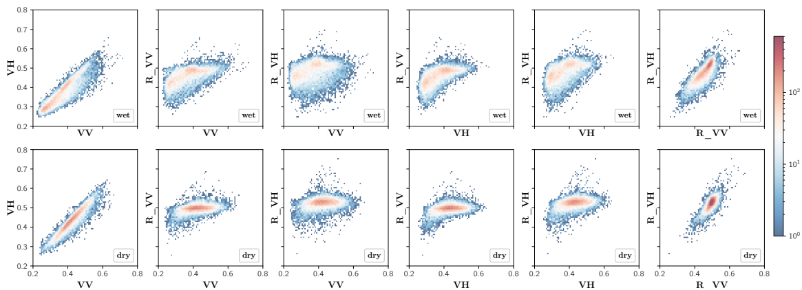
(a) Comparison of the mean for each samples of the four considered channels. The first line of plots corresponds to the wet class and the second to the non-wet class.
