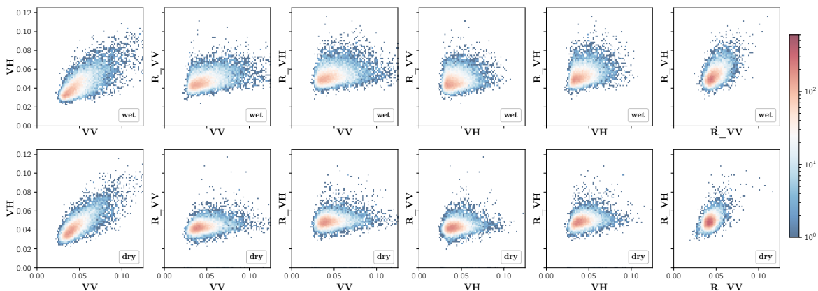
(b) Comparison of the standard deviation for each samples of the four considered channels. The first line of plots corresponds to the wet class and the second to the non-wet class.
