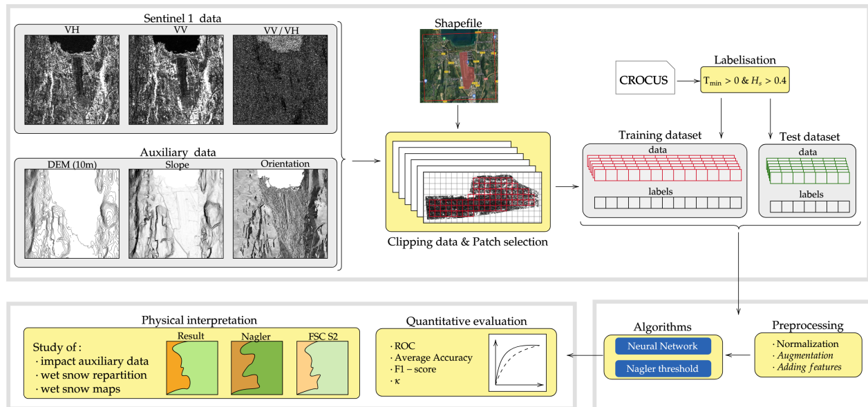
Fig. 1: Diagram of the complete chain for creating a labelled dataset for wet snow detection from SAR and auxiliary data and evaluating the dataset using different algorithms and metrics.
