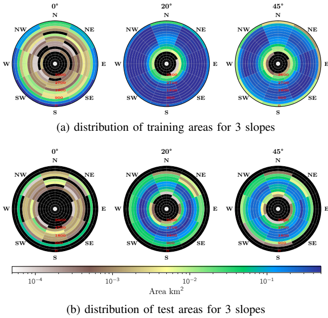
Fig. 5: Topographical distributions of the test and training samples according to the discretisation given by CROCUS, for slope, orientation and elevation
