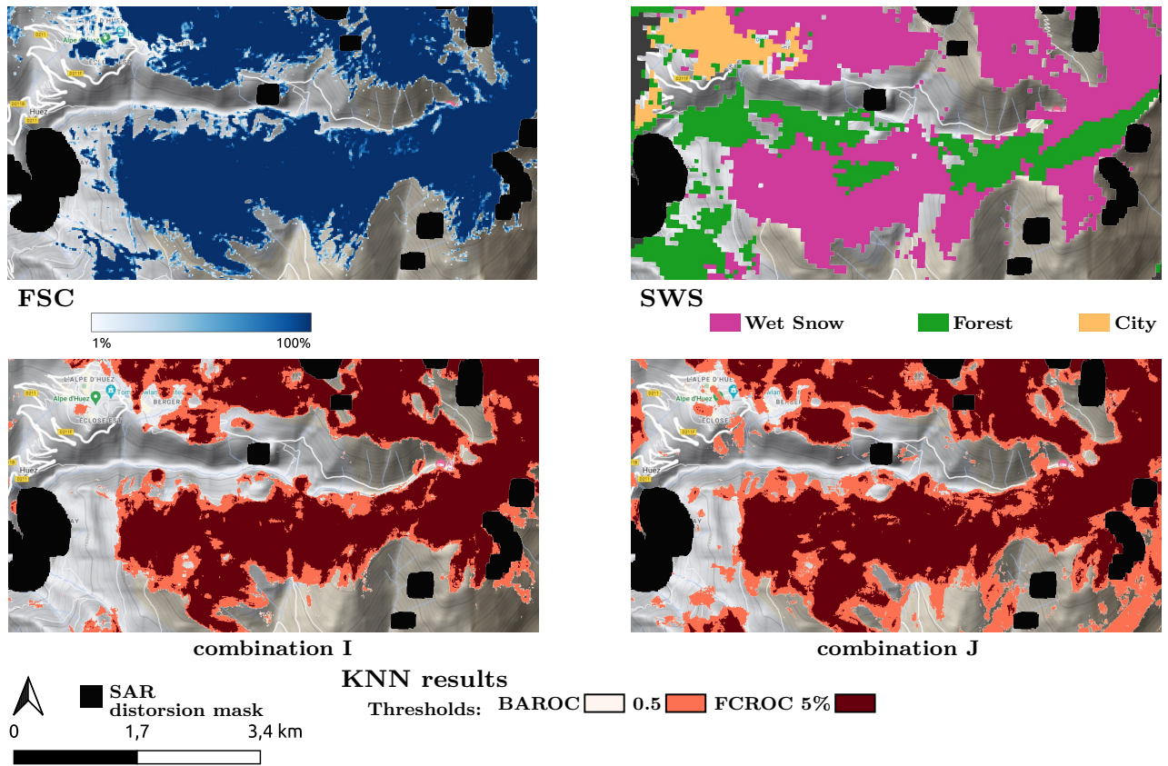
(a) Maps of snow classification results for two dates in comparison with Copernicus FSC and SWS products March 31, 2021
