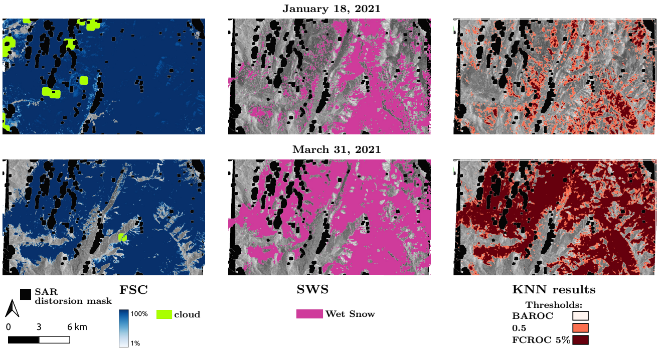
(a) Maps of snow classification results for two dates in comparison with Copernicus FSC and SWS products March 31, 2021
