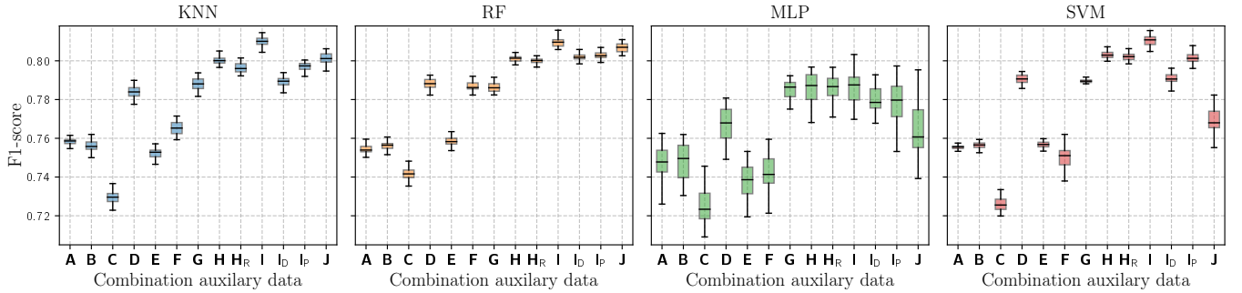
Fig. 7: Evaluation of the F1-score for the 4 best algorithms obtained in Table IV as a function of the combinations of the considered channels
