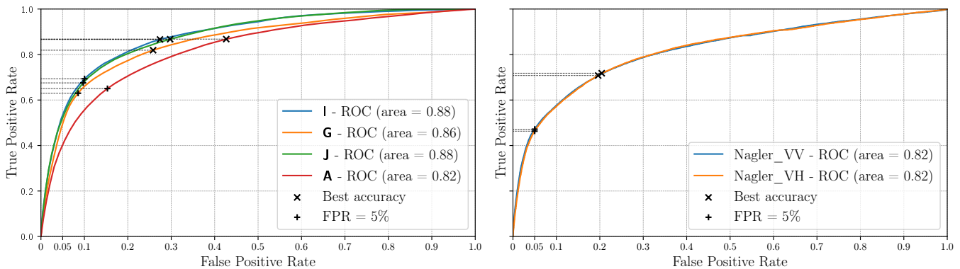
Fig. 8: ROC curve for 4 input channel combinations for the KNN classifier and their associated BAROC and FCROC metric at 5% (left). ROC curve for the simple thresholding type classifier on the mean of each sample for the VV and VH channels (Nagler thresholding), with BAROC and FCROC metrics (right).
