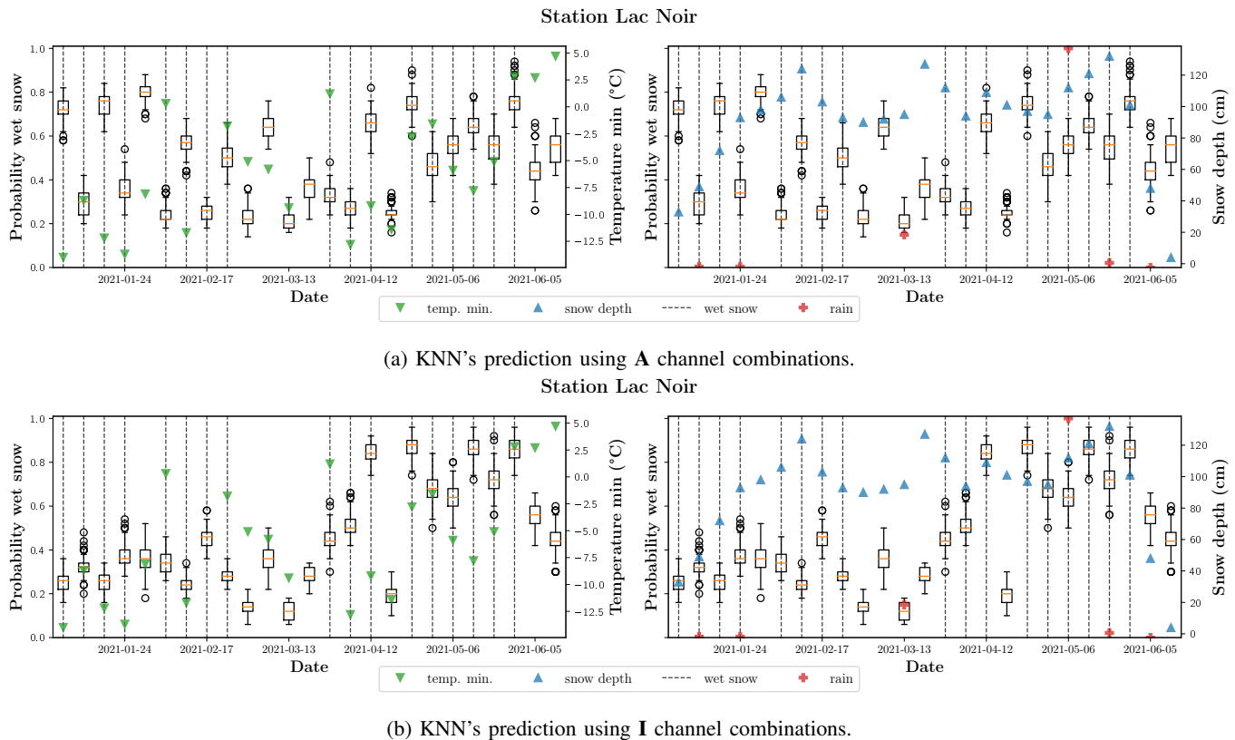
Fig. 13: Comparison of Lac Noir station measurements with KNN's prediction.
