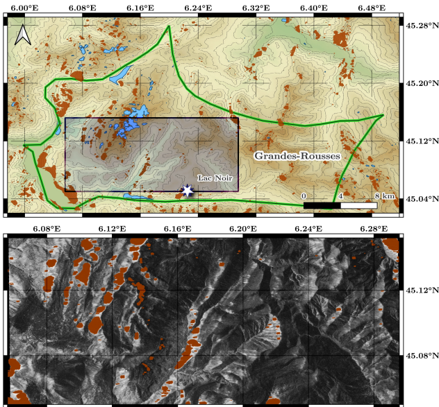
Fig. 3: Position of the validation area (semi-transparent dark blue rectangle and span (\sqrt{VV^2 + VH^2}) of the 2 polarimetrics channels inside the test massif of the Grandes Rousses. The white star represents the station considered for in-situ assessment. Areas affected by the SAR geometric distortions (layover and shadow) are masked in brown.
