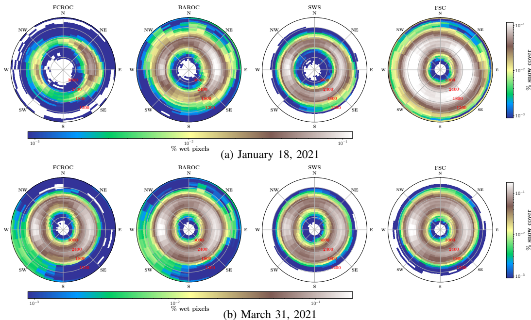
Fig. 12: Diagrams of the distribution of wet pixels (FCROC, BAROC, SWS) and snow cover (FSC) as a function of altitude and orientation for a slope less than 45^\circ , for two dates
