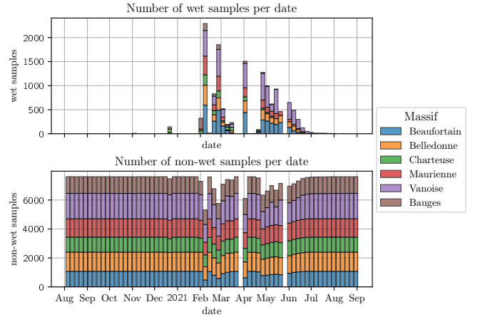
Fig. 6: Distribution of the number of samples between August 2020 and 2021, according to the 6 training massifs considered for the two classes wet and non wet .
