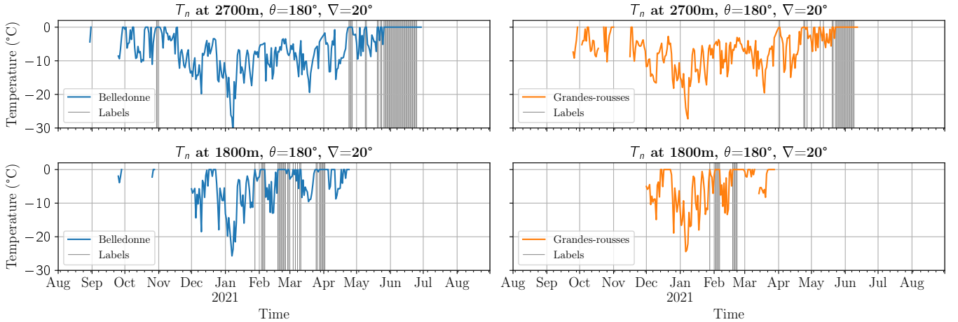
Fig. 4: Minimum snowpack temperature given by CROCUS between August 2020 and 2021. In blue, the curves are given for the Belledonne massif and in orange for the Grandes Rousses massif, for 2 given altitudes, facing south. The grey lines show the dates on which the equation (1) is respected.
