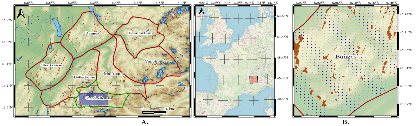
Fig. 2: A. Location of the study area in the French Northern Alps: 6 massifs outlined in red for training and green for testing. The area inside the dark blue rectangle highlights the wet snow validation zone. In blue, the water bodies given by IGN. B. Details of the sampling strategy in the Bauges massif for training. The small blue square represent the sample selection strategy. Layover and shadow are masked in brown.
