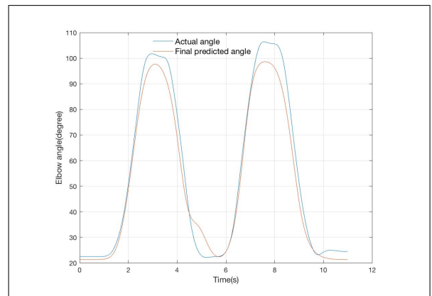
Fig. 10. Testing phase: Measured (blue curve) joint angle and estimated joint angle result of FIS (red curve) in the elbow.
