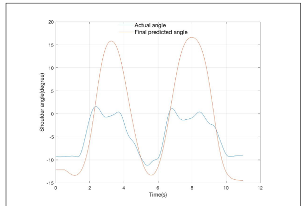
Fig. 9. Testing phase: Measured (blue curve) joint angle and estimated (red curve) joint angle result of FIS in the shoulder.
