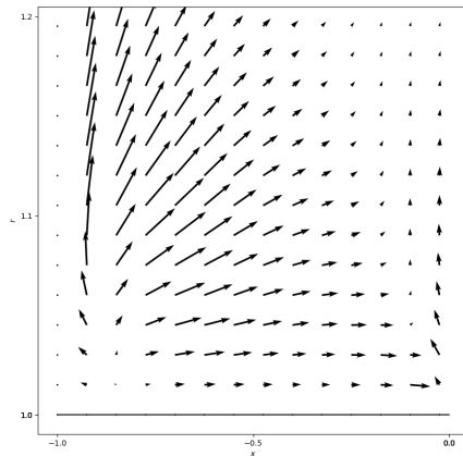
Figure 13: Forcing vectors [\phi_x^{(1)} \ \phi_r^{(1)}]^T atop the nozzle for (S, m, St) = (0, 2, 0) .
