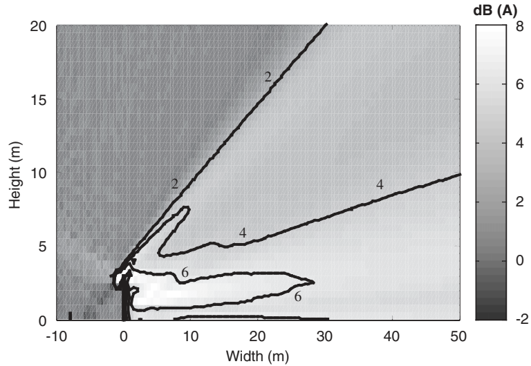
Fig. 13. Map of the efficiency of the multiple-edge crowned barrier with the four optimal parameters. d = 1.02\text{ m} ; \sigma = 10\text{ kPa s m}^{-2} ; h = 0.1\text{ m} ; i = -23^\circ .
