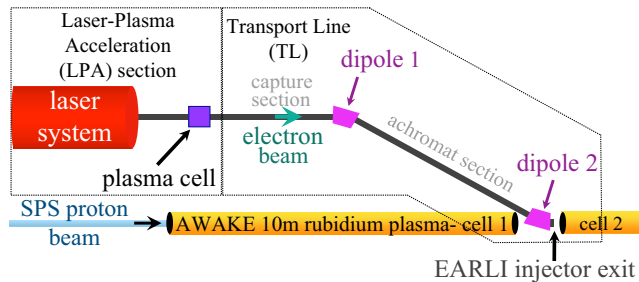
FIG. 1. Schematic layout of the EARLI laser-plasma based electron injector to be insert into the AWAKE environment. The electrons generated in the laser-plasma acceleration section (box on the left) are transported in the transport line (box on the right) up to the gap between the two rubidium plasma cells.
