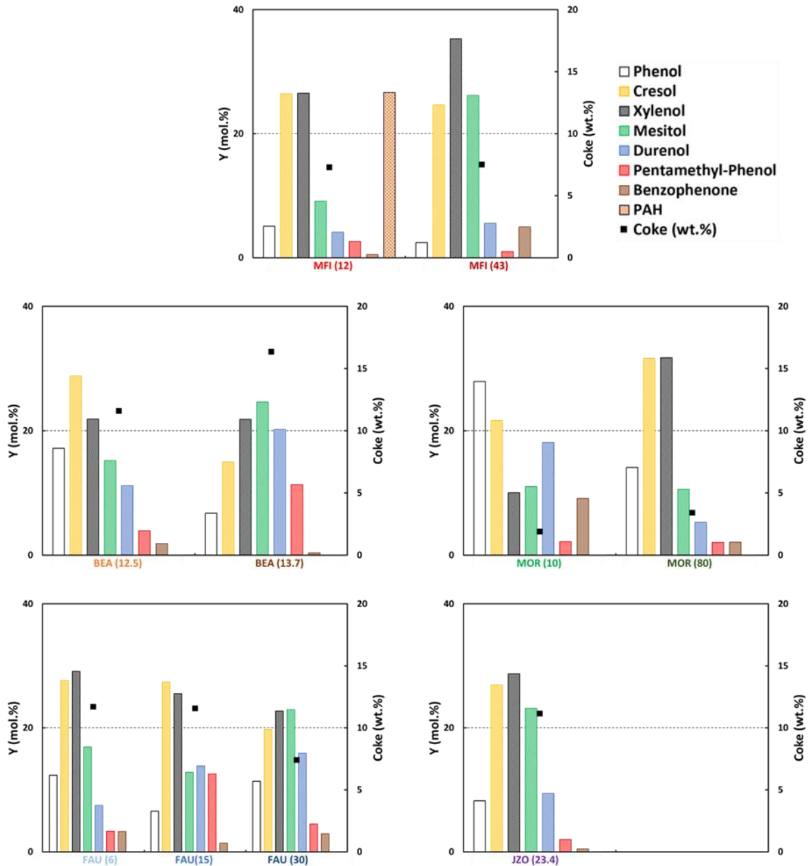
Figure 8: Quantification of the main coke components after 1h of reaction for each catalyst. (Y: fraction of the components in the soluble coke extract).
