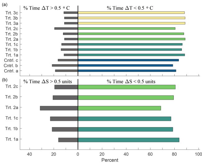
Figure 5. The percentage of time that each mesocosm experienced a deviation greater than (black bars) or less than (colored bars) 0.5 \text{ }^\circ\text{C} ( \Delta T ; a ) or 0.5 in salinity ( \Delta S ; b ) when flow rates were above 2 \text{ L min}^{-1} . “Cntrl.” or “Trt.” are used to refer to the control or treatments, respectively. This excludes the period during which the 90 m pump (12 d) was used but accounts for 42 d out of the 54 d of the experiment. The bar color indicates different treatment groups, as shown on the y axes.
