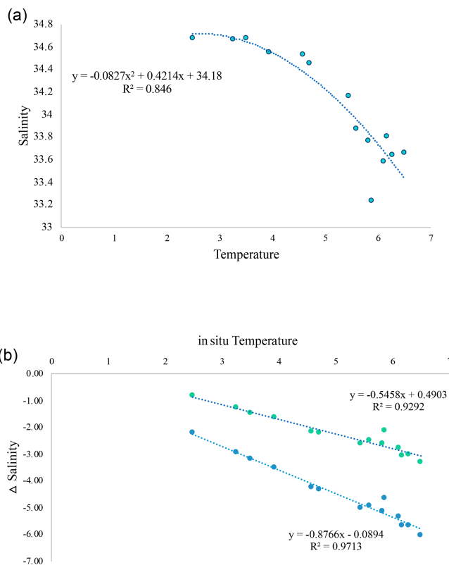
Figure A1. (a) Relationship between temperature and salinity in summer 2020 (weeks 22–35) in Ny-Ålesund, Svalbard. (b) Relationship between estimated delta salinity and in situ temperature, where delta salinity was calculated as the difference between the current mean salinity and the salinity estimated at the temperature increase projected for the SSP2-4.5 (green dots) and SSP5-8.5 (blue dots) scenarios.
