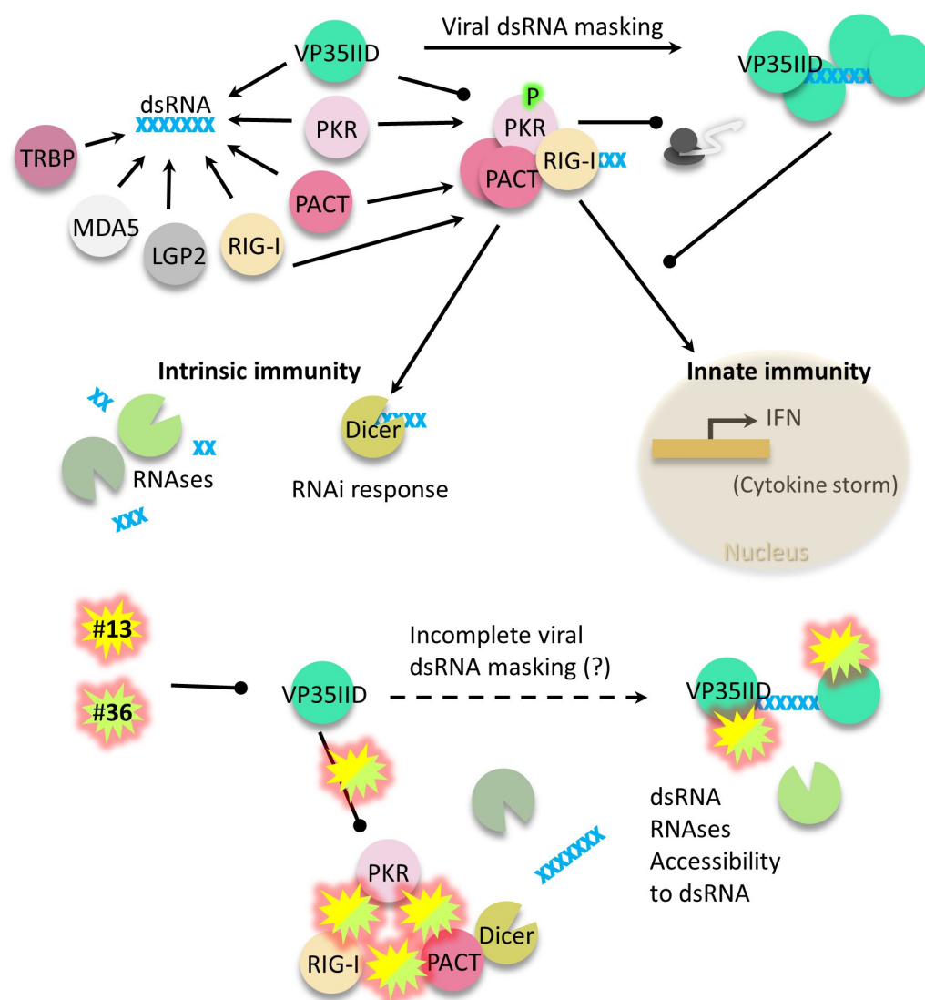
Figure 6. Summary model of the VP35IID crosstalk with dsRNA cell sensors and the effect of compounds #13 and #36. Overall, these compounds restore intrinsic immunity response (immediate degradation of viral dsRNA by RNases and RNAi) without affecting the inhibition of innate immunity by VP35IID, therefore preventing a cytokine storm aggravation. Trans-activation response (TRBP); anti-melanoma differentiation-associated gene 5 (MDA5); Laboratory of Genetics and Physiology 2 (LGP2).
