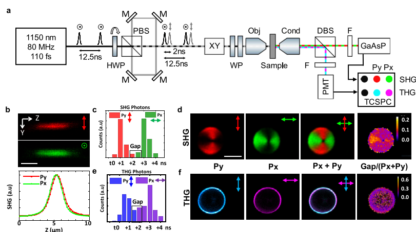
Figure 1. MORPHing setup and characterization. (a) Schematic of the microscope. Pairs of pulses with orthogonal polarization and 2 ns temporal separation are generated by a delay loop. Focused pulses are scanned across the sample. SHG-THG signals corresponding to each polarization state are separated by TCSPC detection. Up to four images are acquired simultaneously. HWP: Half wave plate. PBS: Polarizing beamsplitter. M: Mirror. XY: Galvo scanning. WP: Wave plates. Obj: Objective. Cond: Condensor. DBS: Dichroic beamsplitter. F: Filter. (b) YZ projections of SHG from KTP nanoparticles and axial (Z) profiles. Scale bar: 1 \mu\text{m} . (c) Histogram of SHG photon detection times with the GaAsP detector. (d) Corresponding SHG images of a starch granule. Scale bar: 10 \mu\text{m} . (e) Histogram of THG photon detection times with the PMT detector. (f) THG images of the same starch granule as in (d).
