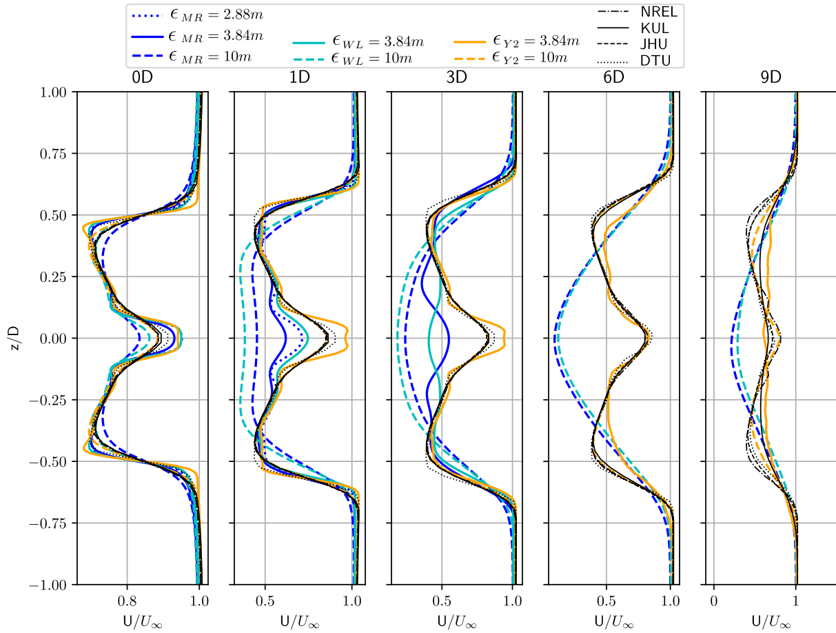
Figure 4: Mean velocity comparison in the wake for all codes.
