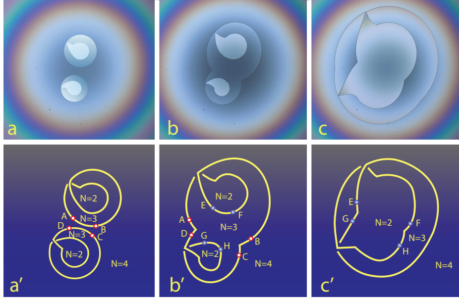
Figure 8. Genesis of the Hopf link. a-a') Nucleation of two folded unknots. b-b') Coalescence of the external loops of the two colliding folded unknots. c-c') Coalescence of the internal loops of the folded unknots.
