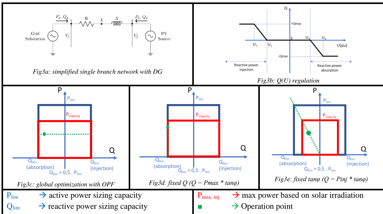
Figure 3: Reactive power control strategies implemented with producer
