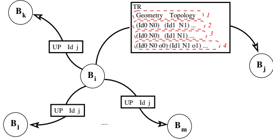
Fig. 5: Summary of the different messages exchanged for the volume transfer operation. There are two types of messages: TR for "TRansfer" and UP for "UPdate other block".
