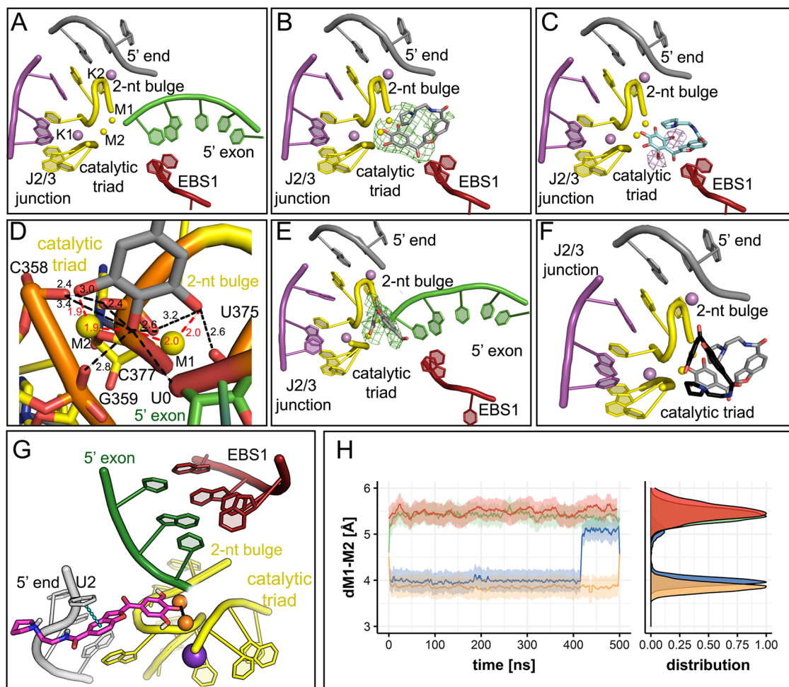
Fig. 4 | Binding of intronistat B to the intron active site after the first step of splicing. A Crystal structure of Oid1-5 with Mg 2+ (yellow spheres), K + (purple spheres), and the 5'-exon-like oligonucleotide 5'-AUUUUAU-3' (green sticks). Active site elements, i.e., the J2/3 junction (magenta), catalytic triad (yellow), 2-nucleotide bulge (yellow), and EB (firebrick) are shown as cartoons. B Crystal structure of Oid1-5 with Mg 2+ , K + , 5'-exon-like oligonucleotide 5'-AUUUUAU-3' (not resolved), and intronistat B (gray sticks) after 1 h soaking. F o - F c electron density omit map calculated before modeling intronistat B, contoured at 3σ, is reported as green mesh. Representation of intronistat B color-coded by crystallographic B-factor is in Supplementary Fig. S27. C Crystal structure of Oid1-5 with Mg 2+ , K + , 5'-exon-like oligonucleotide 5'-AUUUUAU-3' (not resolved), and di-brominated intronistat B derivative ARN25850 (cyan sticks) after 1 h soaking. Violet mesh represents anomalous difference Fourier map contoured at 5σ, revealing bromide atom positions. D Crystal structure of Oid1-5 with Mg 2+ , K + , 5'-exon-like oligonucleotide 5'-AUUUUAU-3', and intronistat B after 2.5 h soaking. Interactions of intronistat B
