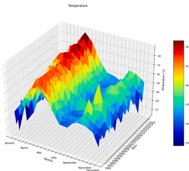
Fig. 9. 3D curves of temperature.
