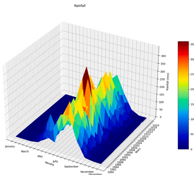
Fig. 10. 3D curves of rainfall.
