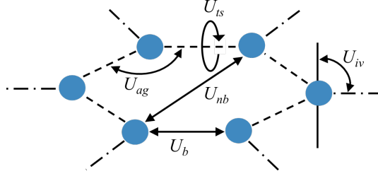
Figure 12: Bond structures and corresponding energy terms of a graphene cell (from [46]).
