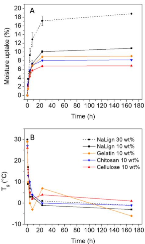
Figure 6. Moisture uptake (A) and T_g values (B) over aging time at 80% RH and 25 °C for various PHU foams loaded with biofillers.
