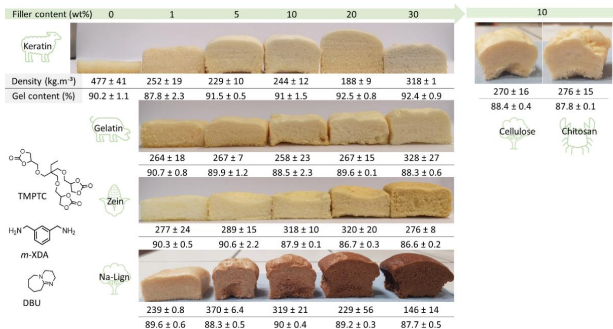
Figure 2. Self-blown NIPU foams prepared from liquid formulations based on TMPTC, m -XDA, DBU and increasing contents of various biofillers: photography, density and gel content of the foams. Foaming was performed at 100 °C for 5 hours.
