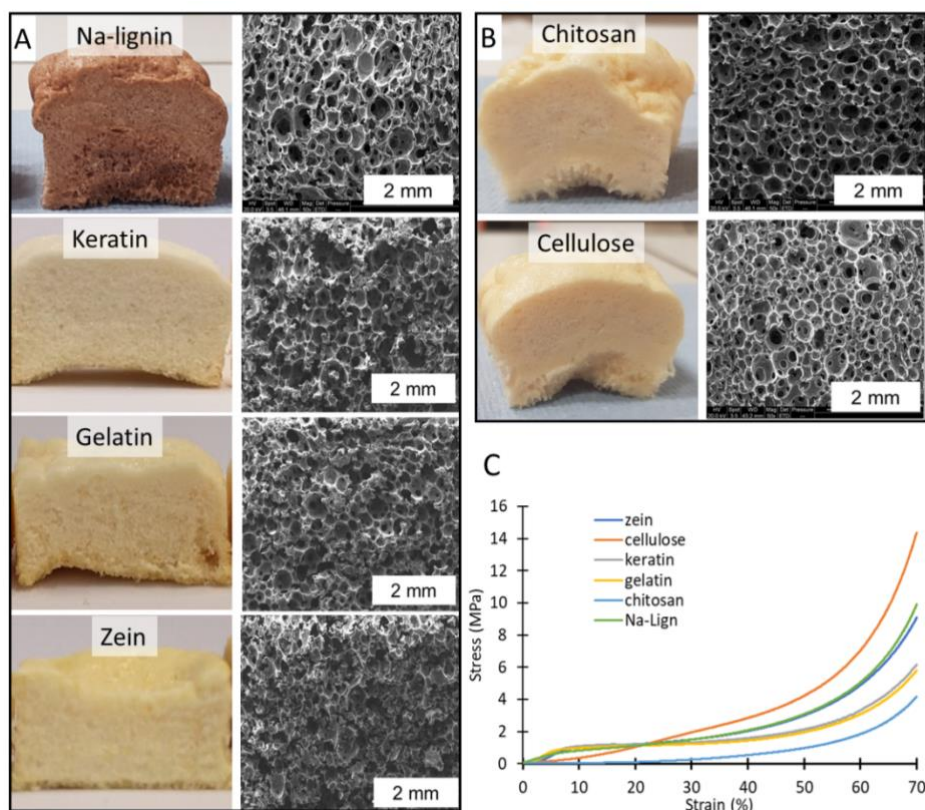
Figure 5. Self-foamed NIPUs with 10 wt% of biofillers. (A and B) Pictures and SEM micrographs, (C) compressive stress-strain curves. See Table 2 for the detailed properties.
