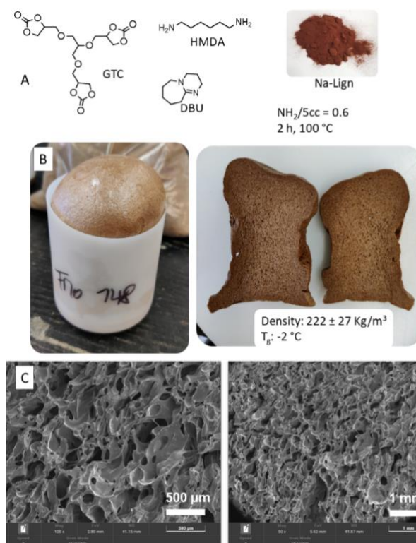
Figure 7. PHU foam of high bio-based content prepared with GTC, HMDA and lignosulfonate catalyzed by DBU (5 mol% vs 5CC). (A) Chemical structures of the precursors, (B) picture of the obtained foam and (C) SEM micrographs.
