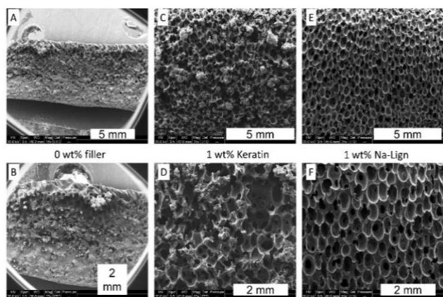
Figure 3. SEM micrographs of foam samples prepared without filler (A, B), with 1 wt% keratin (C, D) or 1 wt% sodium lignosulfonate (E, F). Standard formulations composed of TMPTC, m -XDA ( \text{NH}_2/5\text{CC} = 0.6 ), DBU (5 mol% by respect to 5CC moieties), foamed at 100 °C for 5 h.
