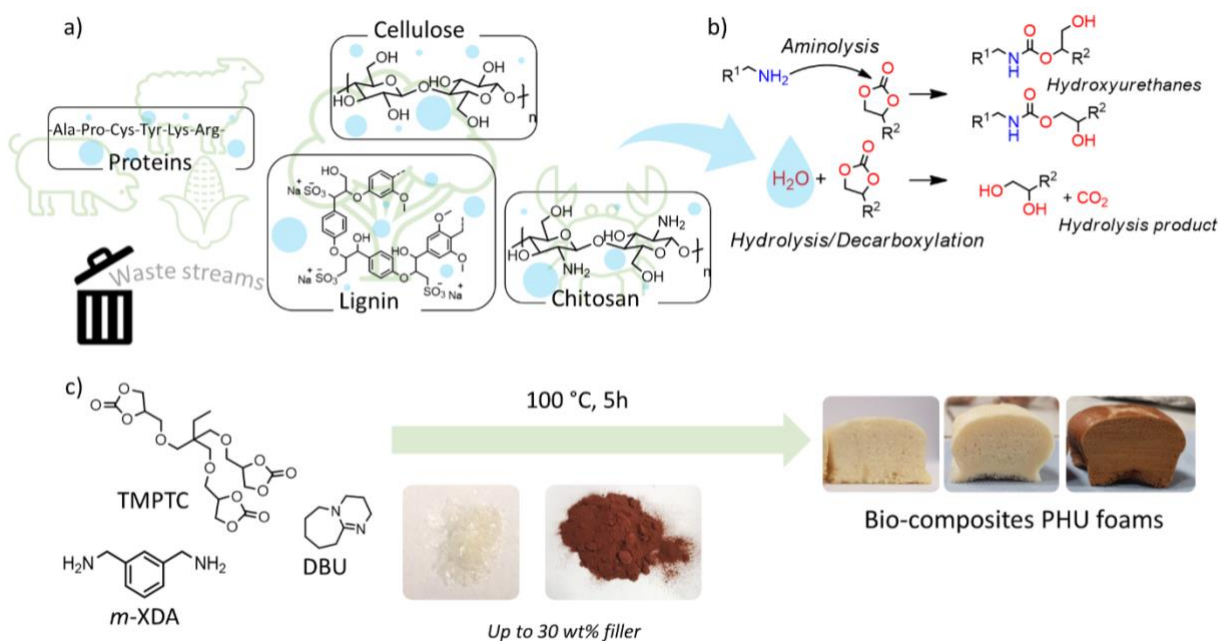
Figure 1. General strategy for the incorporation of waste-biomass into self-foaming isocyanate-free formulations: (A) general chemical structures of the biofillers, (B) reactions for the PHU matrix formation and foaming, (C) example of a typical liquid formulation and its foaming with some representative foams.
