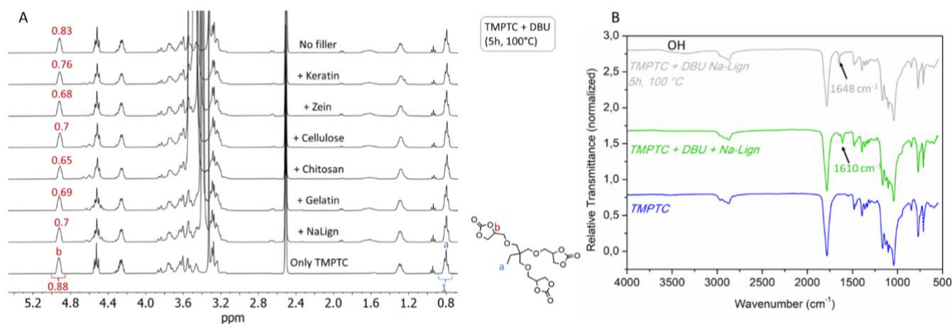
Figure 4. (A) Comparison of the NMR spectra of the TMPTC hydrolysis in the presence of the different biofillers (10 wt%) and DBU for 5 h at 100 °C, and reference NMR spectrum of TMPTC (bottom spectrum). (B) Overlay of FT-IR spectra of TMPTC (blue), TMPTC added by Na-Lign (10 wt%) and DBU before (green) and after reaction at 100 °C for 5 h (grey).
