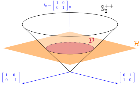
Figure 1. Cone of positive-definite matrices \mathbb{S}_2^{++} in the space of symmetric 2 \times 2 real matrices, and its intersection with the affine hyperplane \mathcal{H} of symmetric 2 \times 2 real matrices with a trace of 2.
