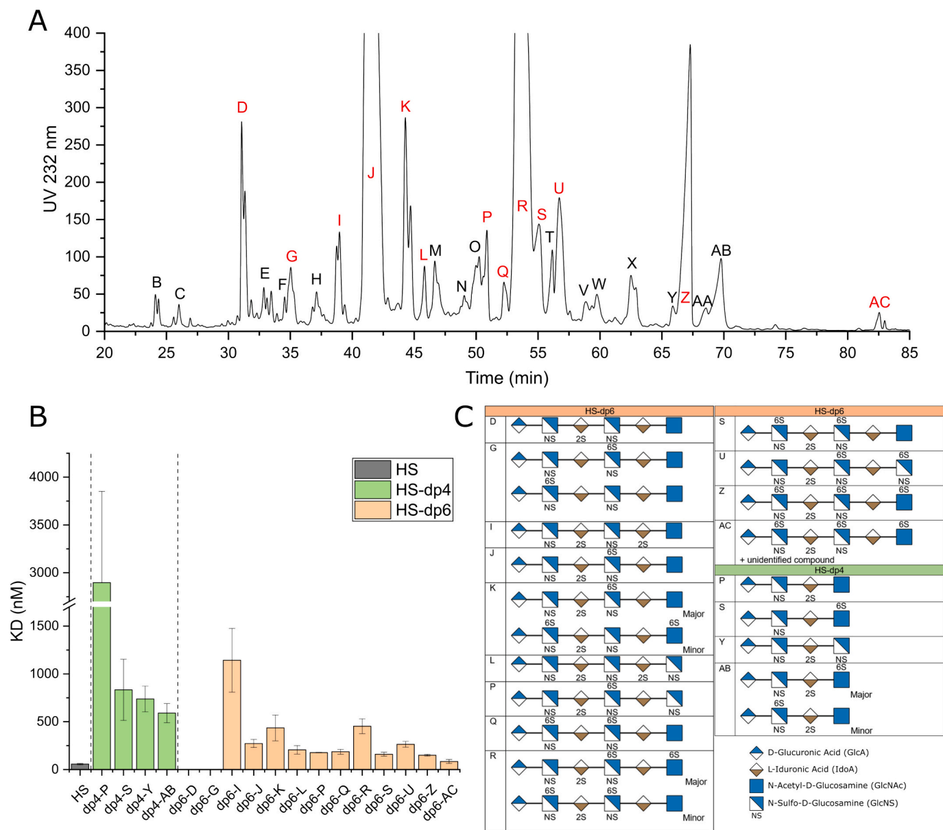
Fig. 4. Characterization of BMP2 binding on HS-oligosaccharides with defined structures.
