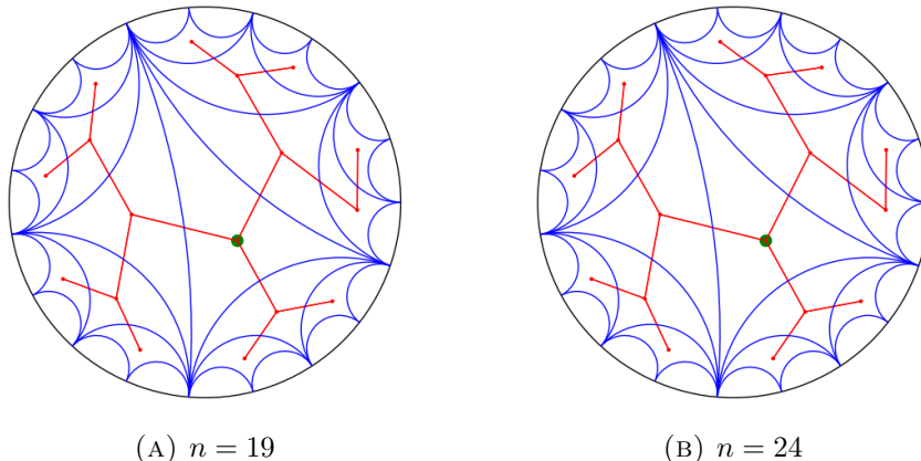
FIGURE 1. Triangulations of ideal n -gons and their dual tree
