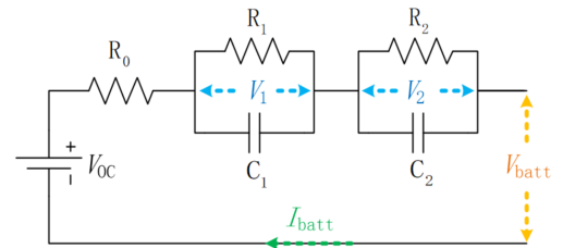
FIG. 3. Double RC circuit Battery model [13]
