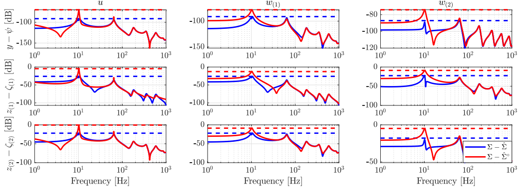
Fig. 3: Bode magnitude plot of error dynamics \Sigma_{lin} - \hat{\Sigma}_{lin}^{\circ} (red) and the error dynamics \Sigma_{lin} - \hat{\Sigma}_{lin} (blue). The horizontal dashed lines indicate the peak error in the correspondingly coloured transfer function.
