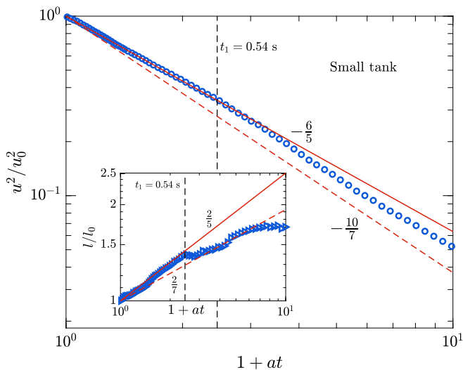
FIG. 2. Decay of the squared velocity fluctuations u^2 as a function of the rescaled time 1 + at (water). The solid line corresponds to a power law defined as (1 + at)^{-6/5} (Saffman) and the dashed line represents the power law (1 + at)^{-10/7} (Batchelor). Inset: time evolution of the integral scale l . The solid line represents the power law (1 + at)^{2/5} (Saffman) and the dashed line (1 + at)^{2/7} (Batchelor).
