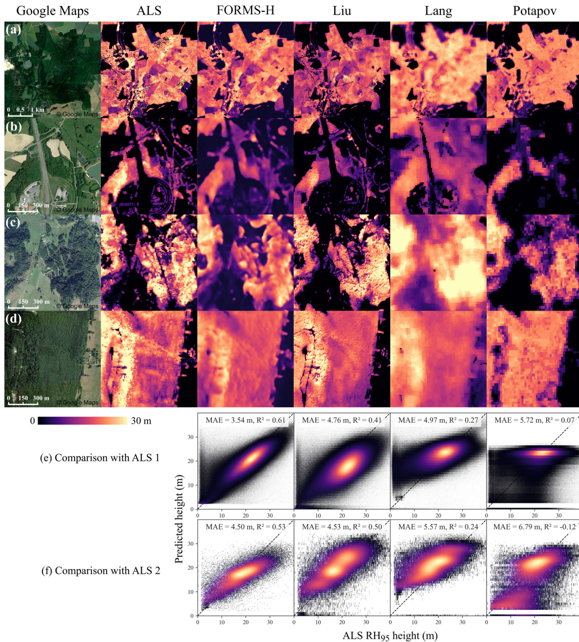
Figure 6. Visual (a, b, c, d) and quantitative (e, f) comparison of ALS RH_{95} height data resampled at 10 m resolution to FORMS-H (10 m resolution) and to three other products at 3 m (Liu et al., 2023), 10 m (Lang et al., 2023), and 30 m resolution (Potapov et al., 2021). Panels (a) comes from ALS 1 data, while (b, c, d) are from ALS 2 data. Panels (a, b) are located on flat terrains. Panels (c, d) are located on steep terrain with 20 to 40° slopes. Panels (e, f) show the comparison with the whole ALS 1 and ALS 2 datasets, in forest pixels filtered with the DLT map (Table 1). The black dashed line is the 1 : 1 line. We applied a uniform noise value in the [-0.5, 0.5] range to the three other height products to allow a better scatterplot density visualization due to the data type provided as integers without changing the performance metrics.
