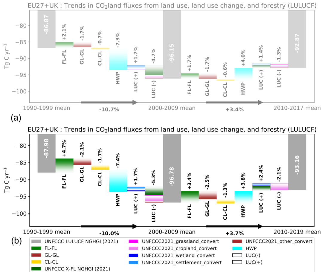
Figure B4. The contribution of changes (%) in CO 2 land fluxes from various LULUCF categories to the overall change in decadal mean for the EU27+UK as reported by member states to the UNFCCC. Panel (a) shows the previous NGHGI data from Petrescu et al. (2021), and panel (b) illustrates data from UNFCCC NGHGI (2021). Changes in land categories converted to other land are grouped to show net gains and net losses in the same column, with the bar color dictating which category each emission belongs to; note that the composition of the “LUC(+)” and “LUC(-)” bars can change between time periods. Not shown are emissions from “Wetlands Remaining wetlands”, “Settlements Remaining settlements”, and “Other land Remaining other land” as none of the BU models used distinguish these categories. The fluxes follow the atmospheric convention, where negative values represent a sink, while positive values represent a source. The color bars are shaded to guide the eye in the direction of the change (white to color).
