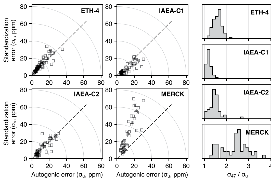
Figure 2. Autogenic vs. standardization errors. Each square marker corresponds to the error components for the average \Delta_{47} value of an unknown sample in each of the InterCarb sessions. Histograms characterize the ratios of total analytical error ( \sigma_{47} ) to autogenic error ( \sigma_u ) for each of the unknown samples.
