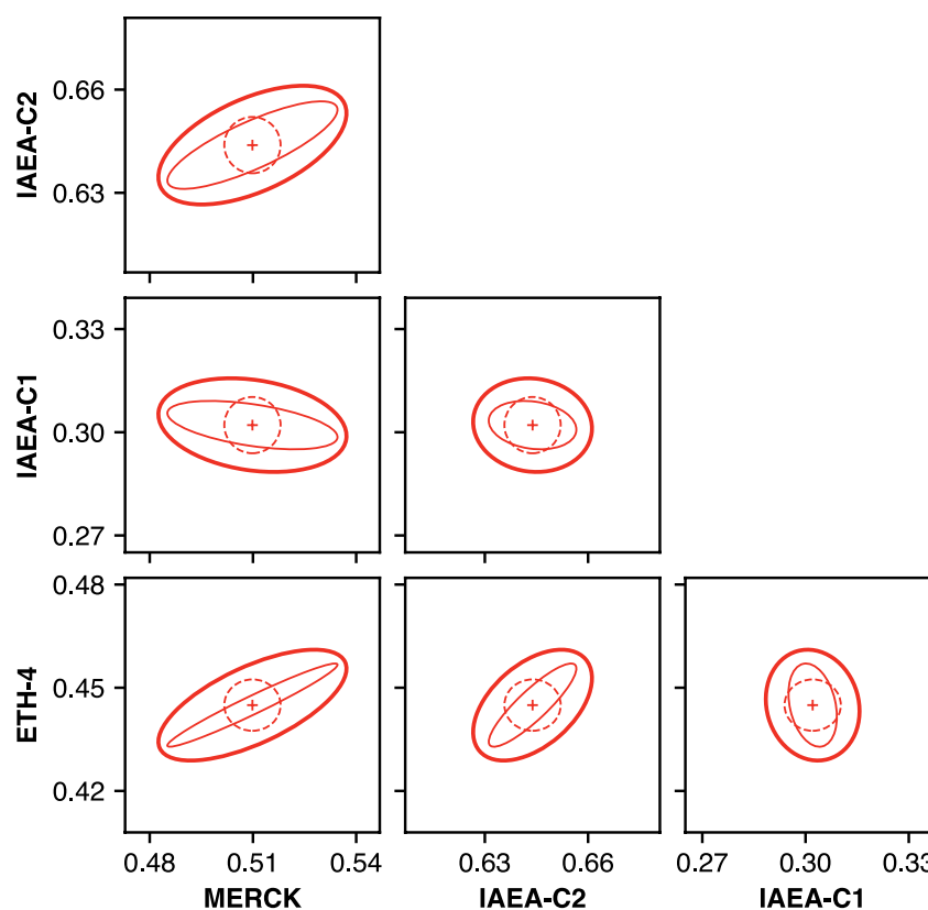
Figure 3. Covariance of errors in session-averaged \Delta_{47} values for unknowns samples. Thick red lines correspond to joint 95% confidence ellipses for the average \Delta_{47} values of each unknown sample in Session02 of Lab12 (cf. upper left panel of Figure 1). Thin red lines and dashed red lines correspond to joint 95% confidence ellipses only taking into account standardization and autogenic errors, respectively.
