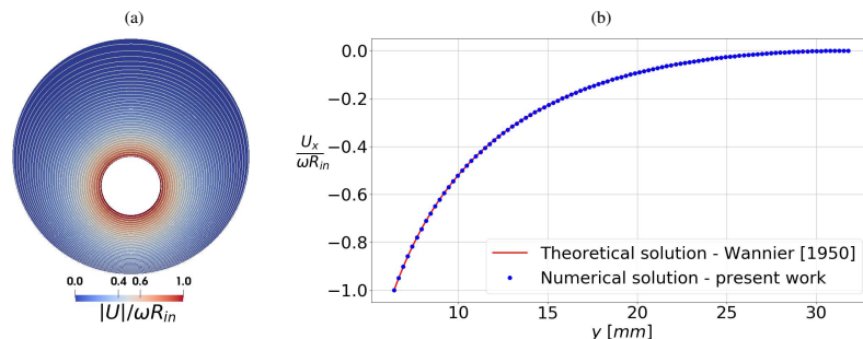
FIG. 4. Flow velocity normalized by the velocity at the inner cylinder \omega R_{in} for \varepsilon = 1/3 : (a) streamlines and velocity norm, (b) azimuthal velocity profile across the large gap along the e_y axis.
