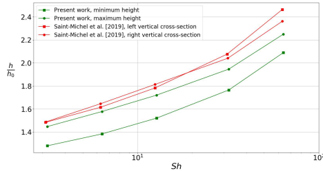
FIG. 25. Resuspension height h calculated at the center of the gap and normalized by the initial sediment height h_0 as a function of the Shields number Sh = \eta_0 \dot{\gamma} / (\rho_p - \rho_f) g a . The red curves correspond to the experimental results of Saint-Michel et al. 3 (right section: circles, left section: squares). The green curves represent the results of the present work for \varepsilon = 0.05 (maximum height: circles, minimum height: squares).
