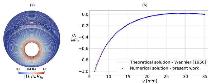
FIG. 5. Flow velocity normalized by the velocity at the inner cylinder \omega R_{in} for \varepsilon = 1/2 : (a) streamlines and velocity vector norm, (b) azimuthal velocity profile across the large gap along the e_y axis.
