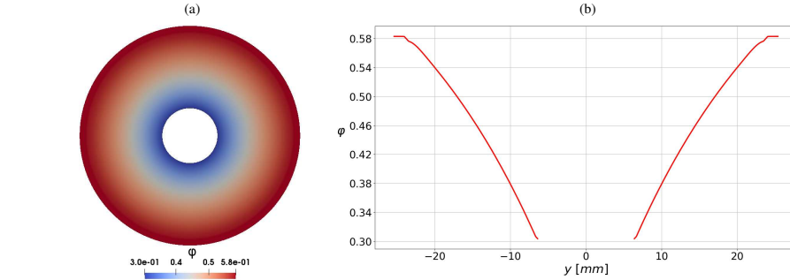
FIG. 9. Computed volume fraction distribution for \varepsilon = 0 at steady state: (a) color map over the whole domain (b) radial profile along the \mathbf{e}_y axis.
