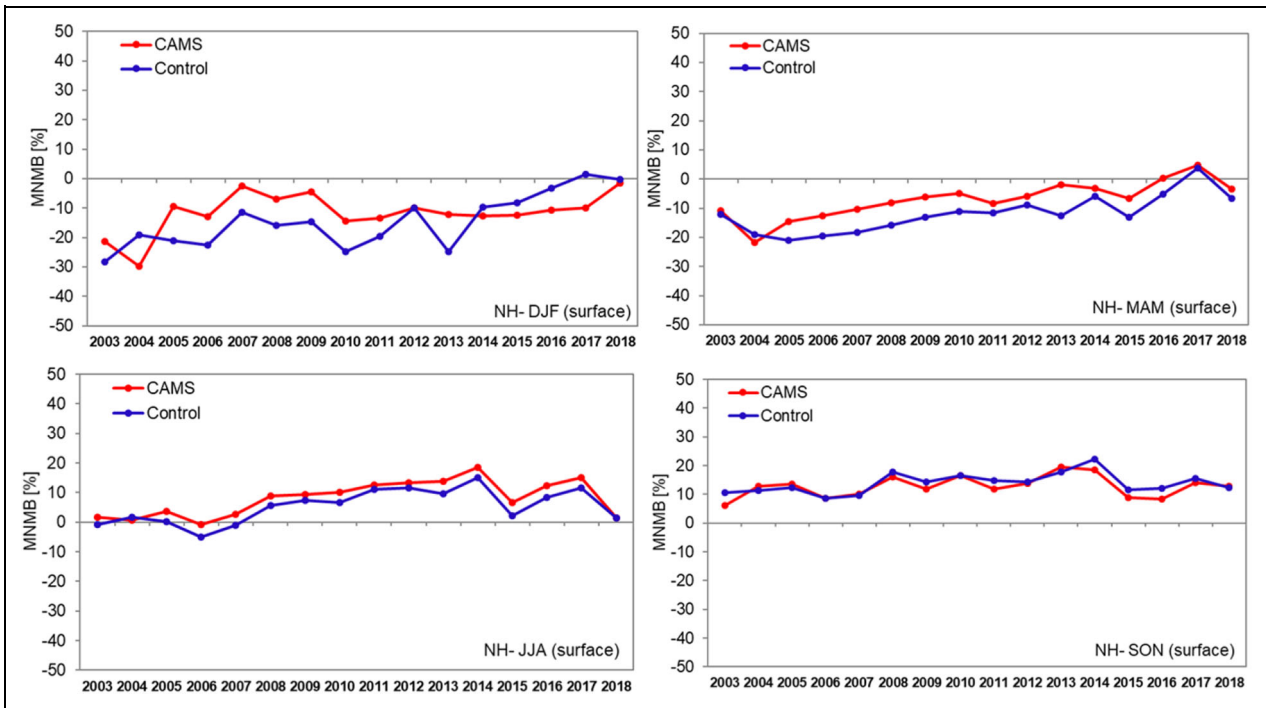
Figure 10. Interannual time series of seasonal MNMBs (%) from the validation with Global Atmosphere Watch surface data for the Northern midlatitudes between 2003 and 2018. Top left: DJF, top right: MAM, bottom left: JJA, bottom right: SON (CAMS reanalysis: red, control run: blue). MNMBs = modified normalized mean biases; CAMS = Copernicus Atmosphere Monitoring Service; DJF = December to February; MAM = March to May; JJA = June to August; SON = September to November. DOI: https://doi.org/10.1525/elementa.2020.00171.f10
