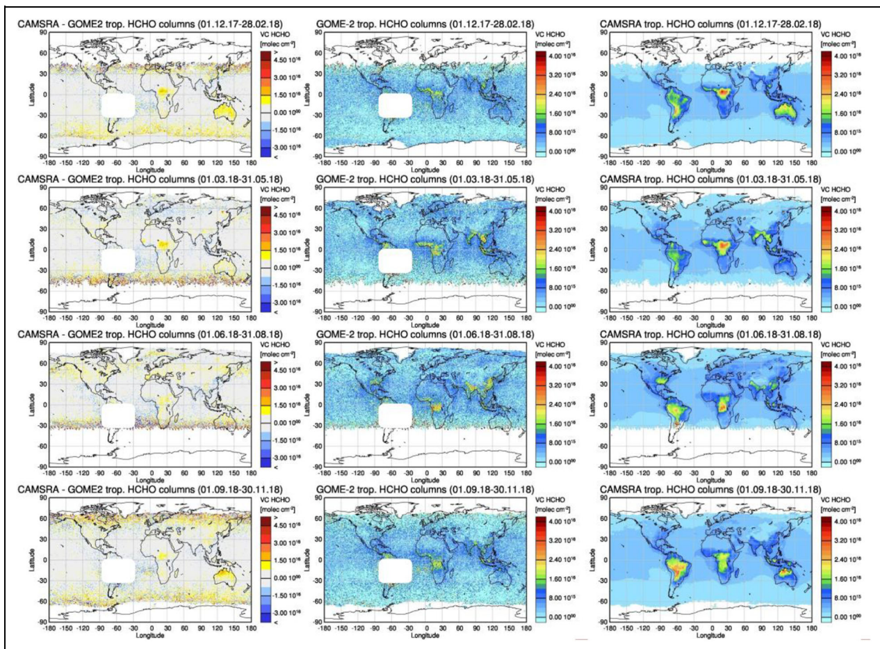
Figure 19. Global map comparisons of satellite-retrieved and model-simulated seasonally averaged tropospheric HCHO columns ( \text{molecule cm}^{-2} ). Satellite-retrieved values in the region of the South Atlantic anomaly are not valid and therefore masked out (white boxes in all images except those that show model results only). HCHO = formaldehyde. DOI: https://doi.org/10.1525/elementa.2020.00171.f19
