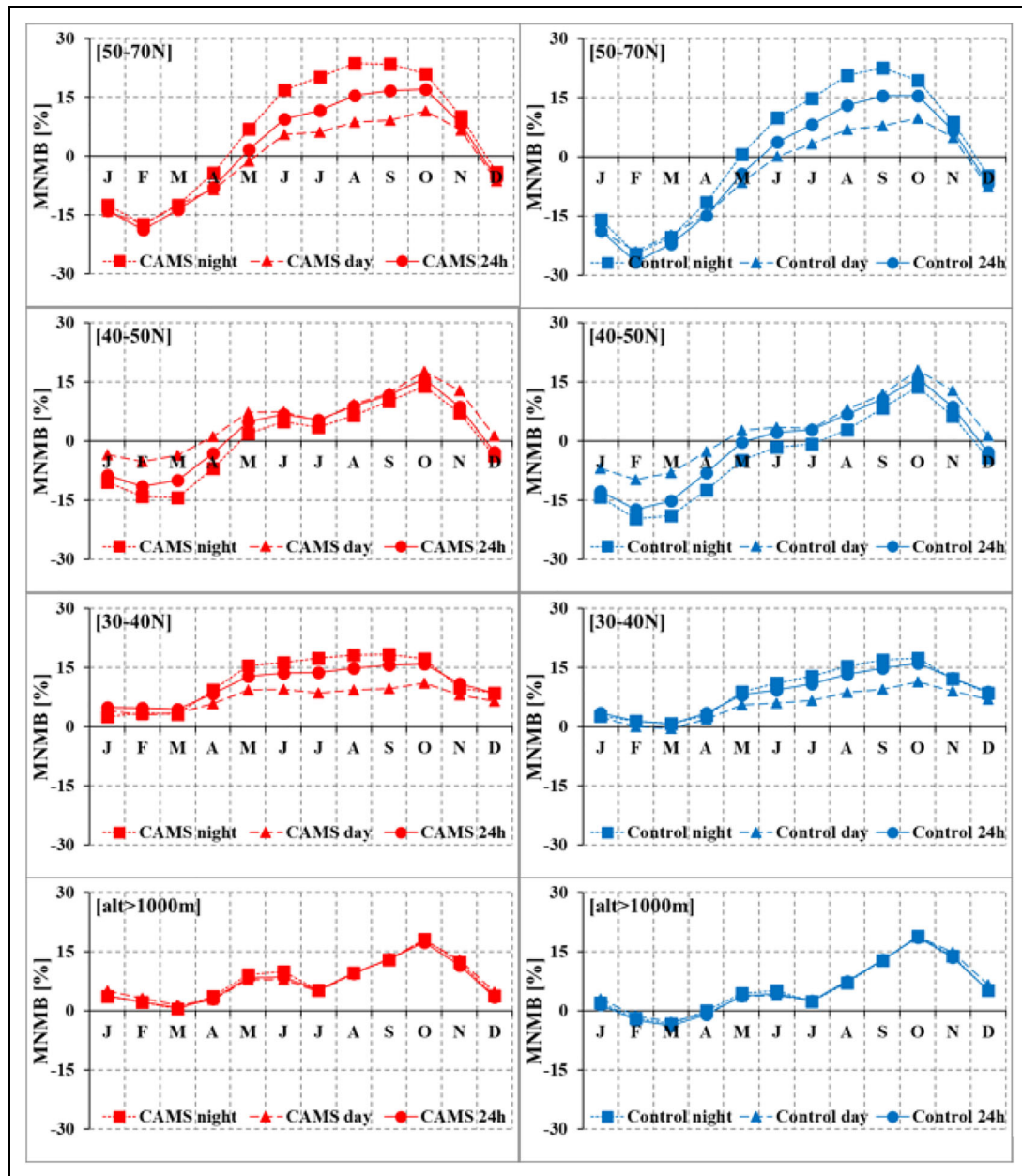
Figure 8. Mean O 3 seasonal variability of MNMBs for the period 2003–2018 from the comparison with European Monitoring and Evaluation Programme surface data. For nighttime (0–3 UTC, squares), for daytime (12–15 UTC, triangles), and for the whole 24 h (circles), over Northern Europe (1st row), Central Europe (2nd row), Southern Europe (3rd row), as well as for stations with an altitude greater than 1,000 m above sea level (4rd row; CAMS reanalysis: red on the left, control run: blue on the right). MNMBs = modified normalized mean biases; CAMS = Copernicus Atmosphere Monitoring Service; UTC = coordinated universal time; O 3 = ozone. DOI: https://doi.org/10.1525/elementa.2020.00171.f8
