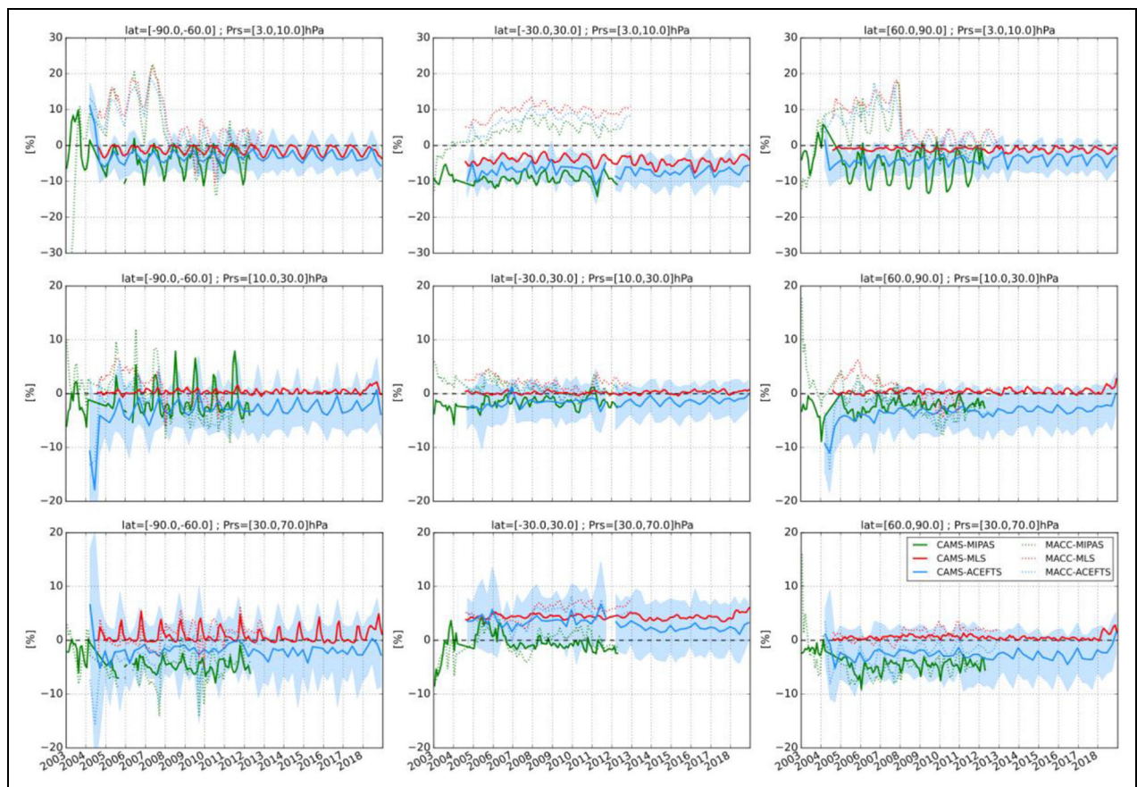
Figure 1. Modified normalized mean bias (MNMB, %) for the O_3 evaluation with satellite data. The time series compares the MNMB of O_3 of the CAMS reanalysis (solid lines) and MACC reanalysis (dotted lines) with observations from MIPAS (green), MLS (red), and ACE-FTS (blue) for the period January 1, 2003, to December 31, 2018, in the upper stratosphere (3–10 hPa mean, top row), middle stratosphere (10–30 hPa mean, middle row), and lower stratosphere (30–70 hPa mean, bottom row) for three latitude bands, respectively: South Pole (90–60°S, left column), Tropics (30°S–30°N, central column), and North Pole (60–90°N, right column). The envelope around the bias between CAMS reanalysis and ACE-FTS represents two normalized standard deviations of the differences. O_3 = ozone; CAMS = Copernicus Atmosphere Monitoring Service; MACC = Monitoring Atmospheric Composition and Climate; MIPAS = Michelson Interferometer for Passive Atmospheric Sounding; MLS = Microwave Limb Sounder; ACE-FTS = Atmospheric Chemistry Experiment-Fourier-Transform Spectrometer. DOI: https://doi.org/10.1525/elementa.2020.00171
