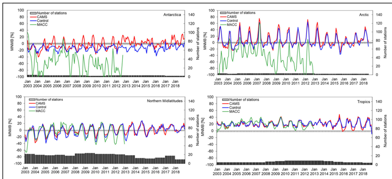
Figure 7. Time series of monthly MNMBs (%) from the comparison against surface O_3 from Global Atmosphere Watch stations between 2003 and 2018. Top left: Antarctica, top right: Arctic, bottom left: Northern midlatitudes, bottom right: Tropics (red: CAMS reanalysis, blue: Control run, green: MAACC reanalysis). MNMB = modified normalized mean biases; CAMS = Copernicus Atmosphere Monitoring Service; MAACC = Monitoring Atmospheric Composition and Climate; O_3 = ozone. DOI: https://doi.org/10.1525/elementa.2020.00171.f7
