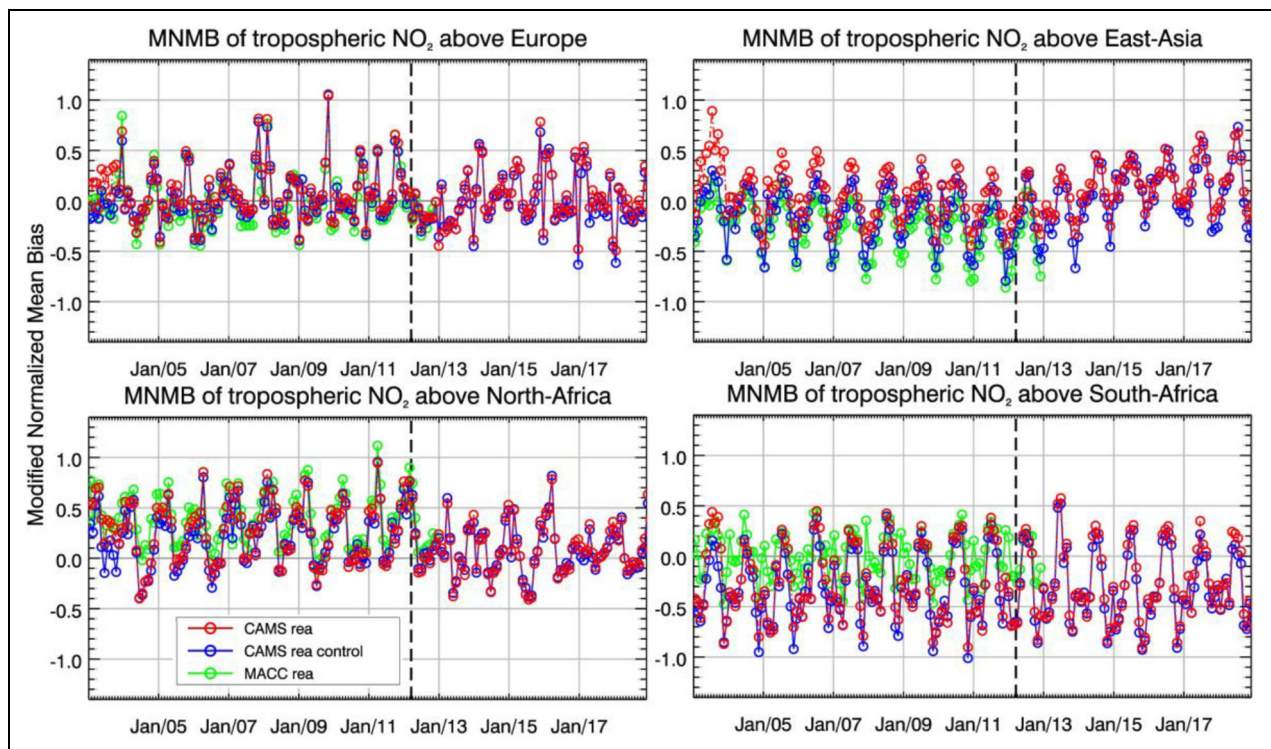
Figure 18. Modified normalized mean bias (MNMB) from the comparison of time series of tropospheric \text{NO}_2 columns from SCIAMACHY and GOME-2 to model results. Results are derived from daily averages over a specific region. Negative daily averages of the retrievals have been flagged in the calculation of the MNMB only. \text{NO}_2 = nitrogen dioxide; SCIAMACHY = Scanning Imaging Absorption Spectrometer for Atmospheric Chartography; GOME = Global Ozone Monitoring Experiment. DOI: https://doi.org/10.1525/elementa.2020.00171.f18
