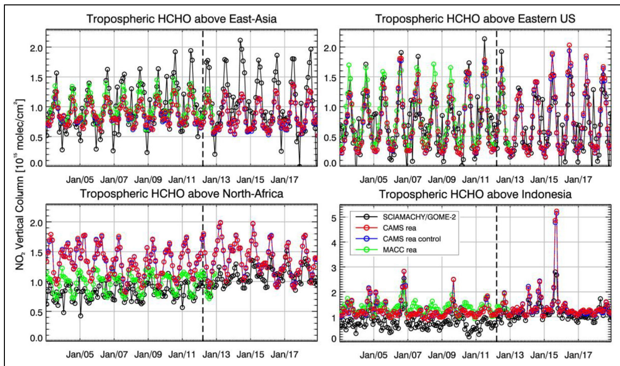
Figure 20. Comparison of time series of tropospheric HCHO columns from SCIAMACHY (up to April 2012) and GOME-2 (from April 2012 onward) to model results (HCHO columns: black, CAMS reanalysis: red, control: blue, and MACC reanalysis: green). The switch from SCIAMACHY to GOME-2 in April 2012 is indicated by the vertical black dashed lines. The regions differ from those used for \text{NO}_2 shown in Figure 17 to better focus on HCHO hotspots: East Asia: 25\text{--}40^\circ\text{N} , 110\text{--}125^\circ\text{E} ; Eastern United States: 30\text{--}40^\circ\text{N} , 75\text{--}90^\circ\text{W} ; Northern Africa: 0\text{--}15^\circ\text{N} , 15^\circ\text{W}\text{--}25^\circ\text{E} ; and Indonesia: 5^\circ\text{S}\text{--}5^\circ\text{N} , 100\text{--}120^\circ\text{E} . Negative satellite-retrieved values over Eastern United States are due to a lack of data during the Northern Hemisphere winter months for this region. HCHO = formaldehyde; SCIAMACHY = Scanning Imaging Absorption Spectrometer for Atmospheric Chartography; GOME = Global Ozone Monitoring Experiment; CAMS = Copernicus Atmosphere Monitoring Service; MACC = Monitoring Atmospheric Composition and Climate; \text{NO}_2 = nitrogen dioxide. DOI: https://doi.org/10.1525/elementa.2020.00171.f20
