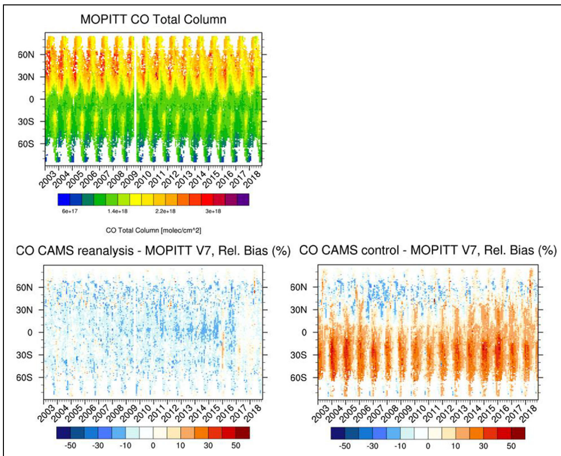
Figure 11. Measurements of Pollution in the Troposphere (MOPITT) V7 CO total column (upper panel) as a function of latitude and time from January 2003 to December 2018. Relative biases between MOPITT V7 and the CAMS reanalysis (lower panel, left) and between MOPITT V7 and the control run (lower panel, right). CAMS = Copernicus Atmosphere Monitoring Service; CO = carbon monoxide. DOI: https://doi.org/10.1525/elementa.2020.00171.f11
