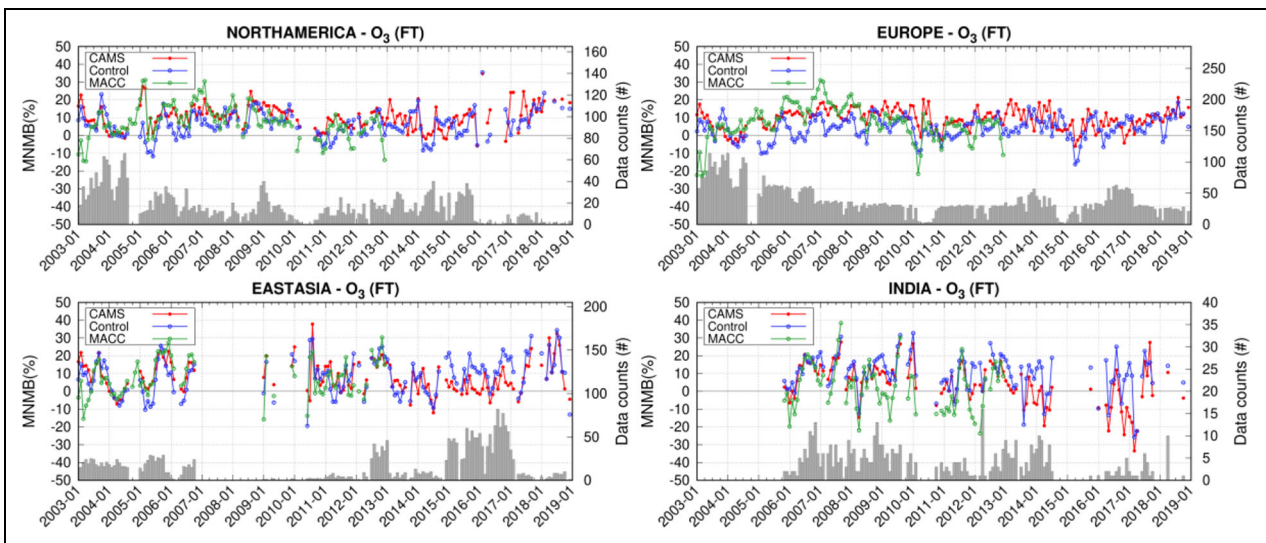
Figure 5. Time series of monthly MNMBs (%) from the comparison against In-service Aircraft for a Global Observing System O 3 aircraft data in the free troposphere for the period 2003–2018. Top left: North America, top right: Europe, bottom left: East Asia, bottom right: India. The plots show averages over various airports in the free troposphere (350–850 hPa) for the CAMS reanalysis (red), control run (blue), and MACC reanalysis (green). MNMBs = modified normalized mean biases; CAMS = Copernicus Atmosphere Monitoring Service; MACC = Monitoring Atmospheric Composition and Climate; O 3 = ozone. DOI: https://doi.org/10.1525/elementa.2020.00171.f5
