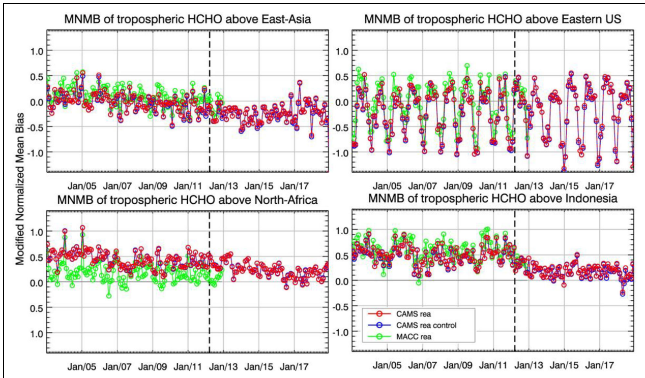
Figure 21. Time series of MNMBs (derived from daily averages) from the comparison of tropospheric HCHO columns from SCIAMACHY (up to April 2012) and GOME-2 (from April 2012 onward) to model results (CAMS reanalysis: red, control: blue, and MACC reanalysis: green). Negative daily averages of the retrievals have been flagged in the calculation of the MNMB only. MNMBs = modified normalized mean biases; HCHO = formaldehyde; SCIAMACHY = Scanning Imaging Absorption Spectrometer for Atmospheric Chartography; GOME = Global Ozone Monitoring Experiment; CAMS = Copernicus Atmosphere Monitoring Service; MACC = Monitoring Atmospheric Composition and Climate; MNMB = modified normalized mean bias. DOI: https://doi.org/10.1525/elementa.2020.00171.f21
