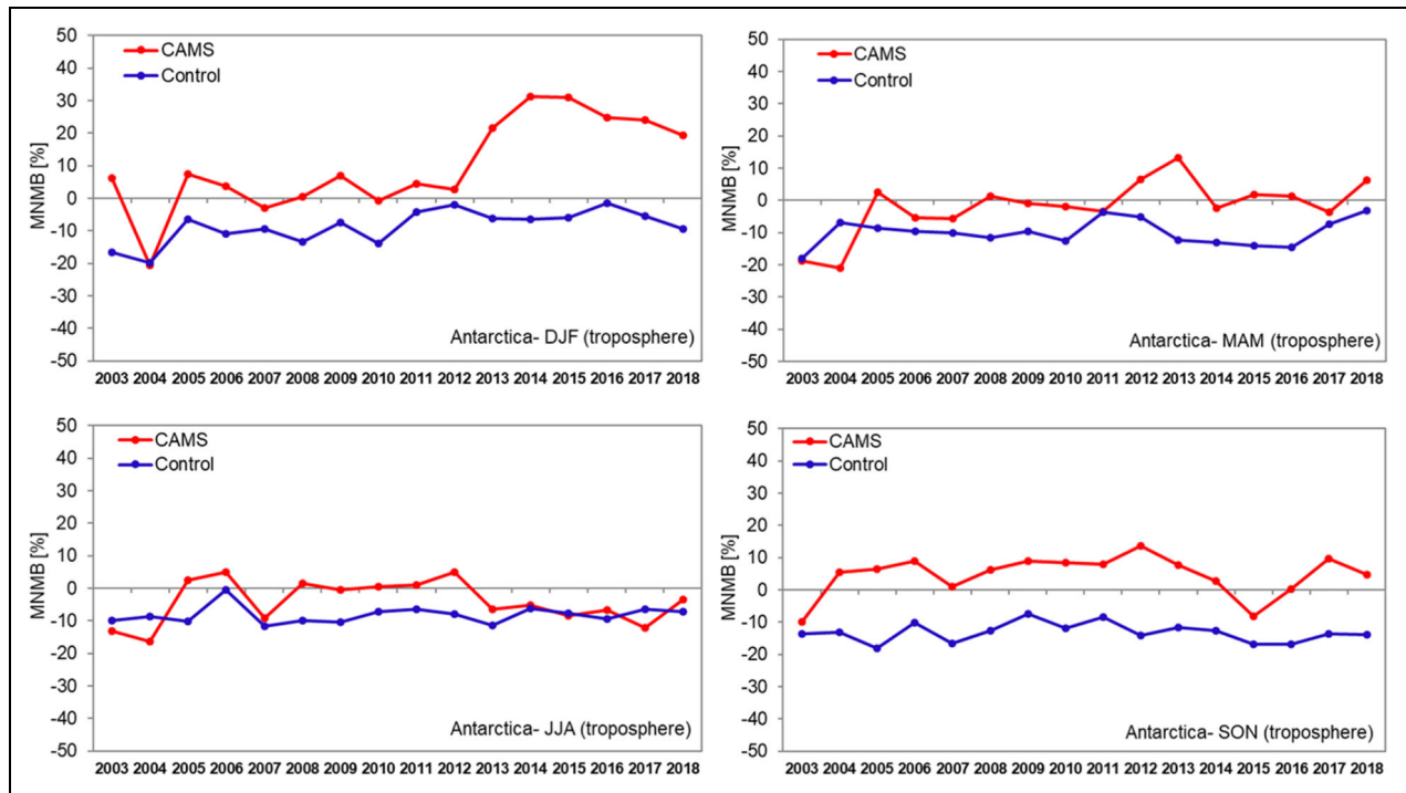
Figure 6. Interannual time series of seasonal MNMBs (%) from the validation with ozonesondes in the free troposphere for Antarctica between 2003 and 2018. Top left: DJF, top right: MAM, bottom left: JJA, bottom right: SON (CAMS reanalysis: red, control run: blue). MNMBs = modified normalized mean biases; CAMS = Copernicus Atmosphere Monitoring Service; DJF = December to February; MAM = March to May; JJA = June to August; SON = September to November. DOI: https://doi.org/10.1525/elementa.2020.00171.f6
