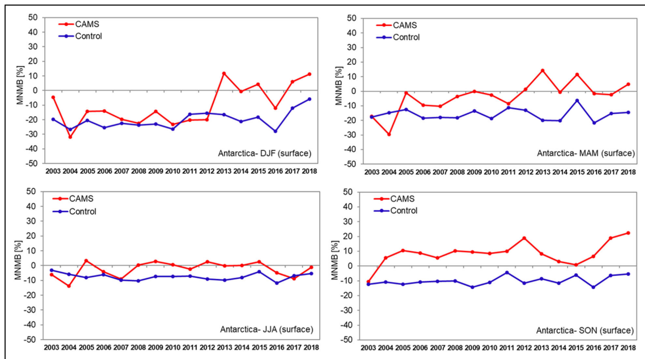
Figure 9. Interannual time series of seasonal MNMBs (%) from the validation with Global Atmosphere Watch surface data for Antarctica between 2003 and 2018. Top left: DJF, top right: MAM, bottom left: JJA, bottom right: SON (CAMS reanalysis: red, Control run: blue). MNMBs = modified normalized mean biases; CAMS = Copernicus Atmosphere Monitoring Service; DJF = December to February; MAM = March to May; JJA = June to August; SON = September to November. DOI: https://doi.org/10.1525/elementa.2020.00171.f9
