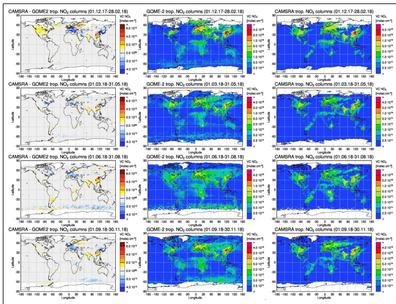
Figure 16. Global map comparisons of satellite-retrieved and model-simulated seasonally averaged tropospheric \text{NO}_2 columns ( \text{molecule cm}^{-2} ). From top to bottom: DJF 2017/2018, MAM 2018, JJA 2018, and SON 2018. The difference between CAMS reanalysis and GOME-2 is shown in the left, GOME-2 in the middle, and the CAMS reanalysis in the right column. GOME-2 data were gridded to model resolution (i.e., 0.75^\circ \times 0.75^\circ ). Model data were treated with the same reference sector subtraction approach as the satellite data. SON = September to November; DJF = December to February; MAM = March to May; JJA = June to August; \text{NO}_2 = nitrogen dioxide; CAMS = Copernicus Atmosphere Monitoring Service; GOME = Global Ozone Monitoring Experiment. DOI: https://doi.org/10.1525/elementa.2020.00171.f16
