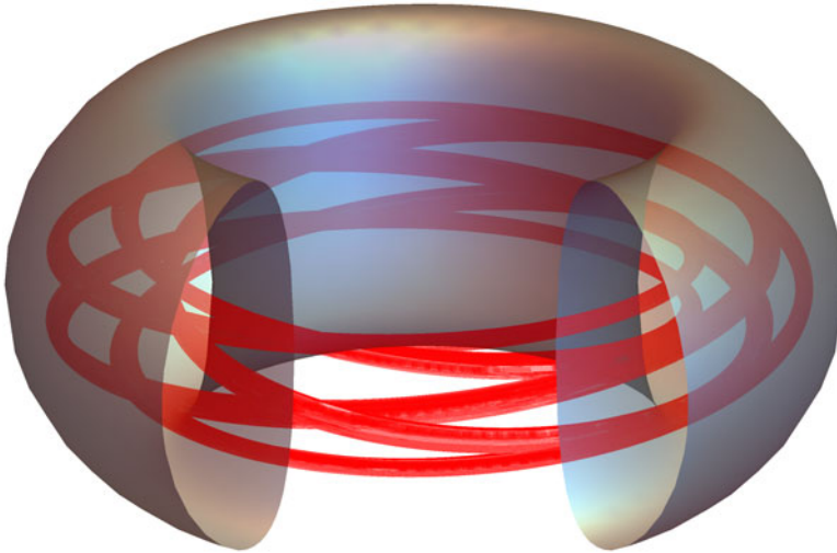
FIGURE 2. When there exists some \psi_J^* such that q(\psi_J^*) = m_0/n_0 , i.e. the mode (m_0, n_0) is resonant for \mathbf{J} , then a current filament flows within the current ‘flux tubes’ attached to elliptic surfaces. In the representation, m_0 = 5 and n_0 = 3 .
