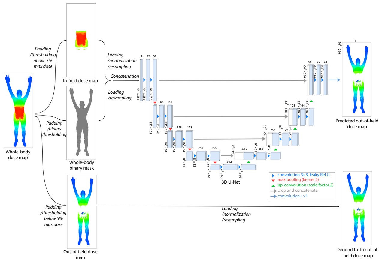
Fig. 1. Dose map preprocessing pipeline and comprehensive design of the implemented 3D U-Net. Dose maps are displayed using logarithmic scale.
