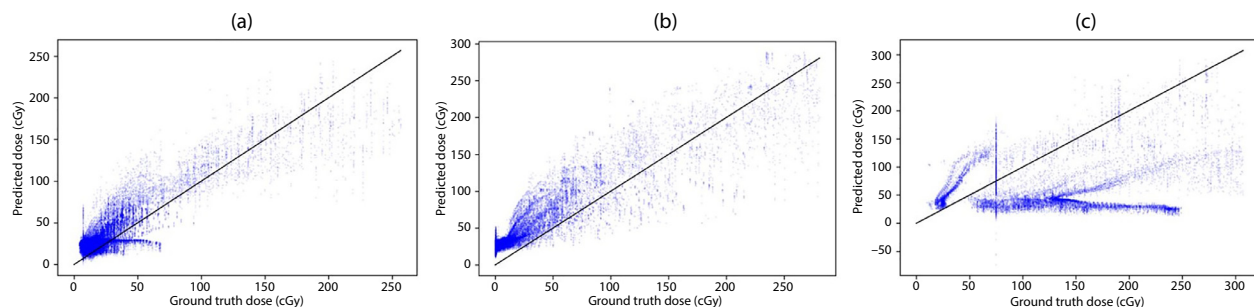
Fig. 5. Doses predicted by the 3D U-Net as a function of the ground truth doses. Each point corresponds to a voxel wise dose evaluation. Scatter plots were drawn for patient a (a), patient b (b), and patient c (c).
