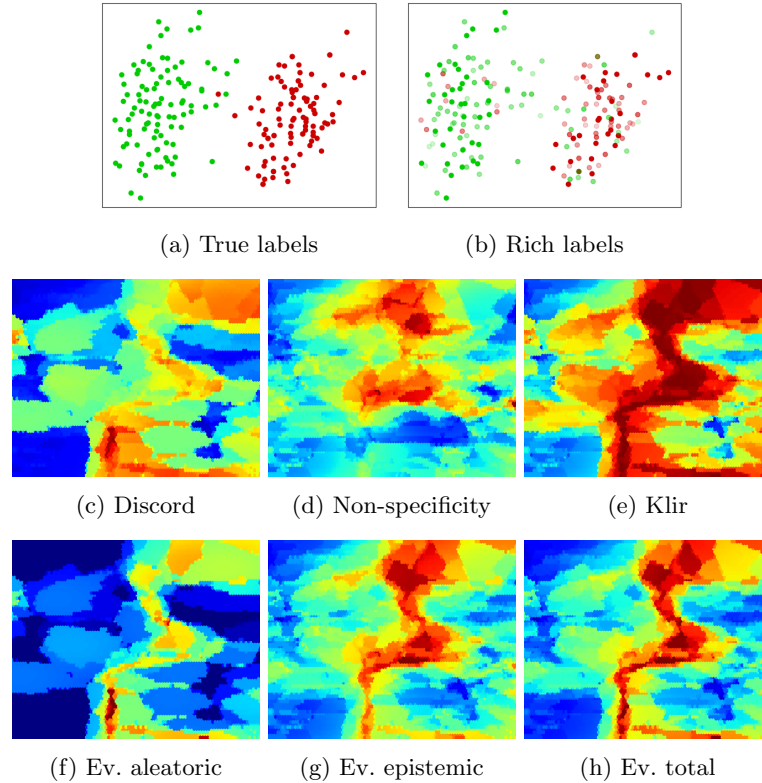
Fig. 10: Ignorance mapping in the Credal Dog-2 dataset: Brittany breed (green) and Beagle breed (red).
