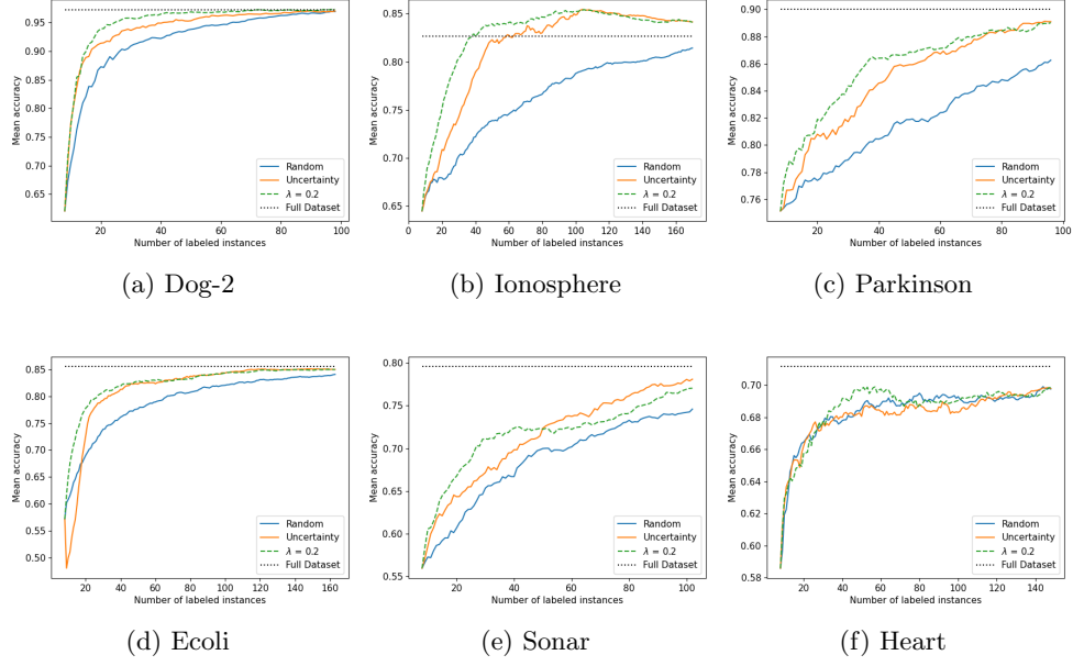
Fig. 11: Mean accuracy vs. number of labeled instances for Random Sampling, Uncertainty Sampling, and the proposed method with \lambda = 0.2 for 6 datasets.
