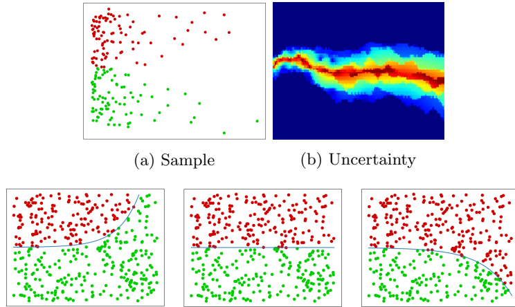
Fig. 4: Visualization of model uncertainty and sample evolution in two-class datasets.
