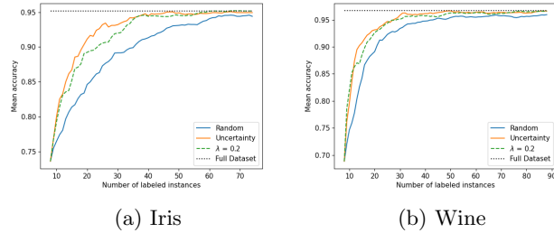
Fig. 12: Mean accuracy vs. number of labeled instances for Random Sampling, Uncertainty Sampling, and the proposed method with \lambda = 0.2 for Iris and Wine.
