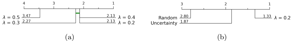
Fig. 13: Critical difference diagrams for different values of \lambda on the proposed method 13a and for random sampling, uncertainty sampling and the proposed method 13b.
