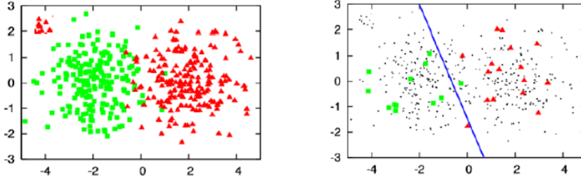
Fig. 1: Illustrating the exploration-exploitation dilemma in active learning: complete dataset vs. active learning iterations.
