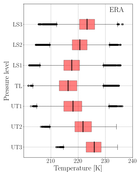
Figure 2. Vertical profile of temperature (K) for IAGOS (blue) and ERA (red).
